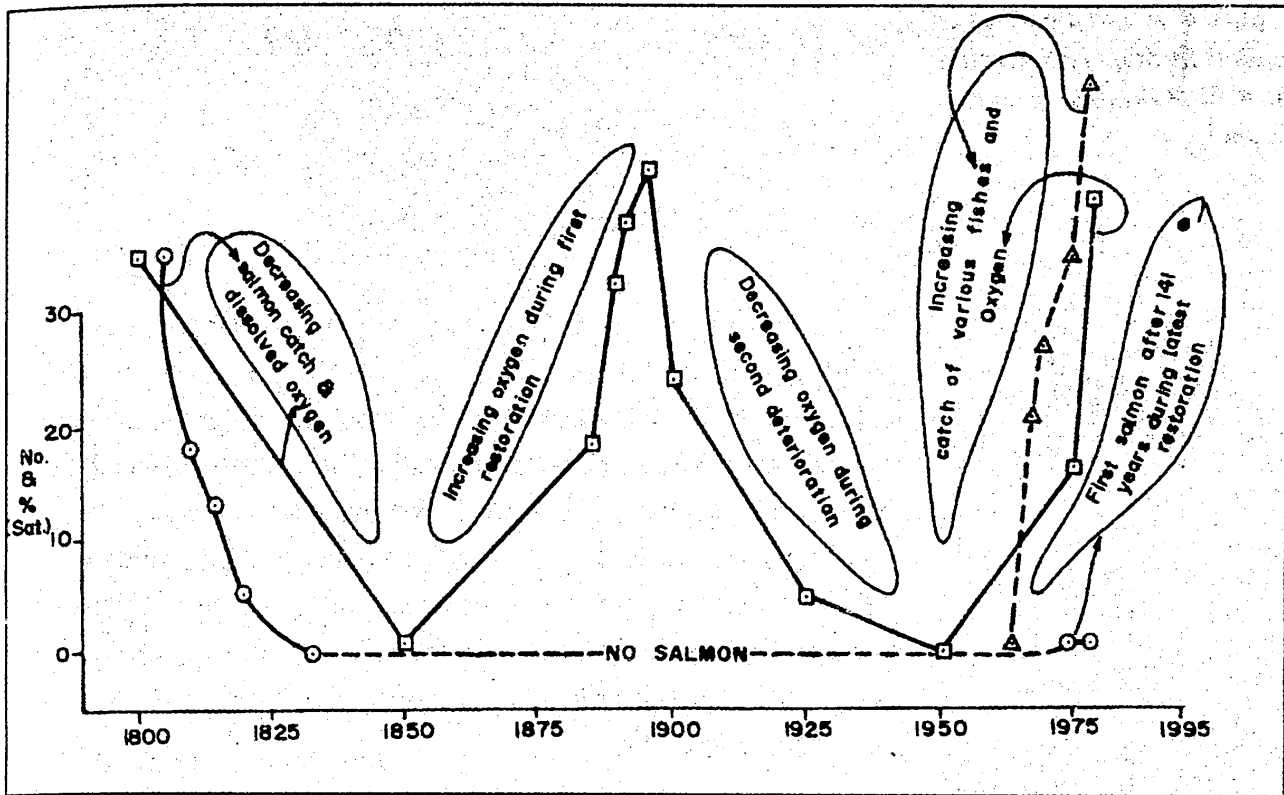
Figure 5. A composite of oxygen saturation levels and fish catch in tidal Thames for about two centuries.
