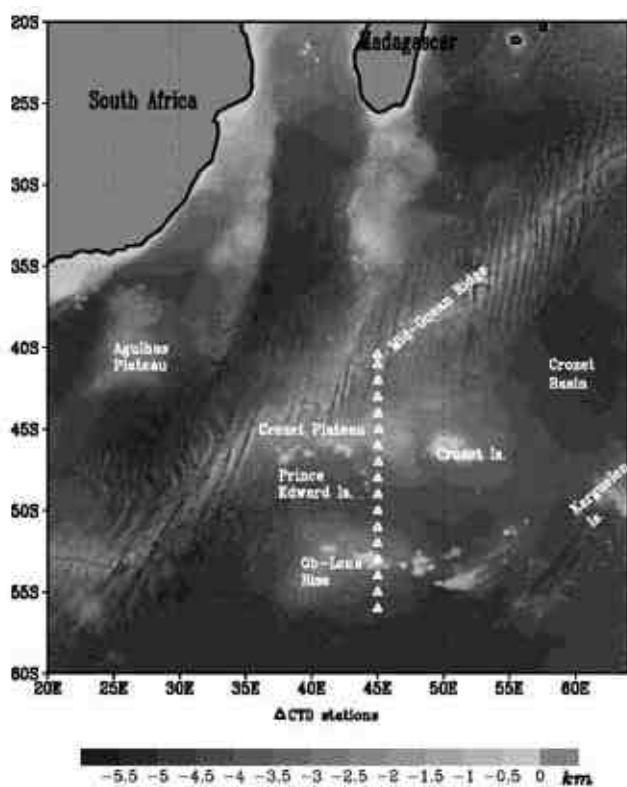
Figure 1. CTD station locations that were occupied (from south to north) during 6–17 February 2004.
