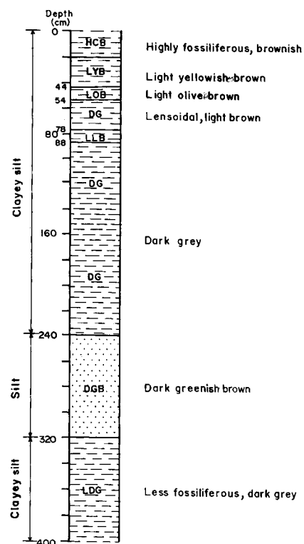
Figure 2. Litholog of the box core-1 as observed onboard.
