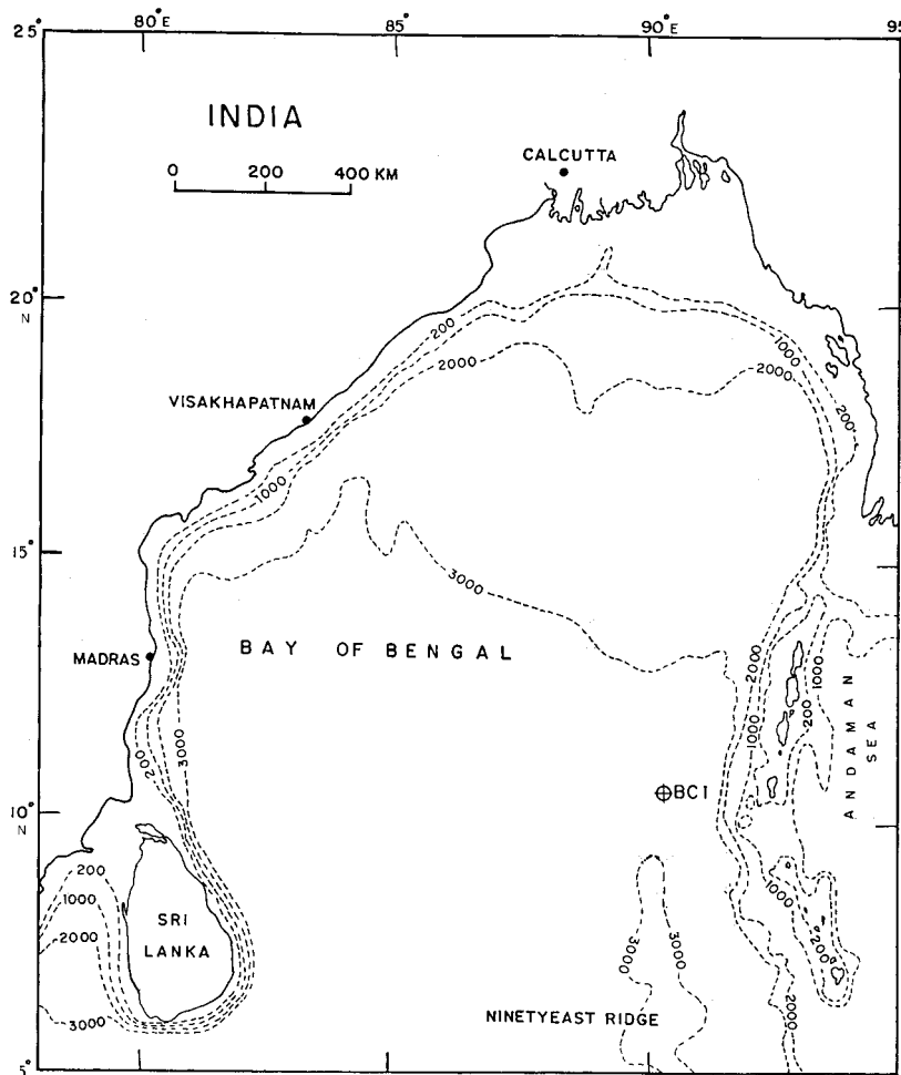
Figure 1. Map showing location of the core sample (BC-1) collected from the Lower Bengal Fan.
