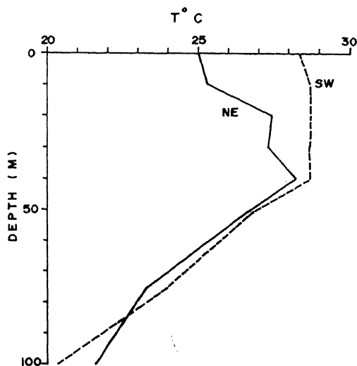
Figure 8. Vertical variation in temperature (°C) in the uppermost 100m at 18° 57' N and 88° 44' E (the circled station in Figure 1). The solid (dashed) curve shows conditions during northeast (southwest) monsoon using data collected during December 1991 (July–August 1989).
