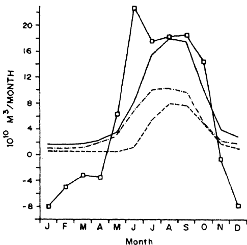
Figure 2. Monthly-mean freshwater influx ( 10^{10} \text{ m}^3/\text{month} ) to the northern Bay. Ganges (---), Brahmaputra (.....) and sum of the two (—); data source; ref. 22. Integral of monthly-mean precipitation minus evaporation over the region north of 14^\circ \text{ N} in the Bay is shown by —□—□—; data source: ref. 10.
