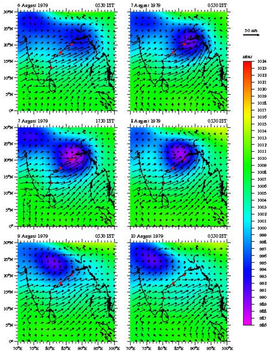
Figure 1 a . Atmospheric pressure at mean sea level and winds at 10 m during Event 1. The 3 red circles mark the location, from north to south, of the 3 tide-gauge stations, Paradip, Visakhapatnam, and Chennai. On 5 August 1979, the remnant of a typhoon moved across central Myanmar (Burma) and appeared over north-eastern Bay of Bengal as a well-marked low-pressure area. It turned into a depression centered at 21°N, 90°E on the morning of 6 August, becoming a deep depression the same evening. It intensified rapidly into a severe cyclonic storm on the morning of 7 August and crossed the north Orissa coast later that day; it weakened and moved westward subsequent to landfall.
