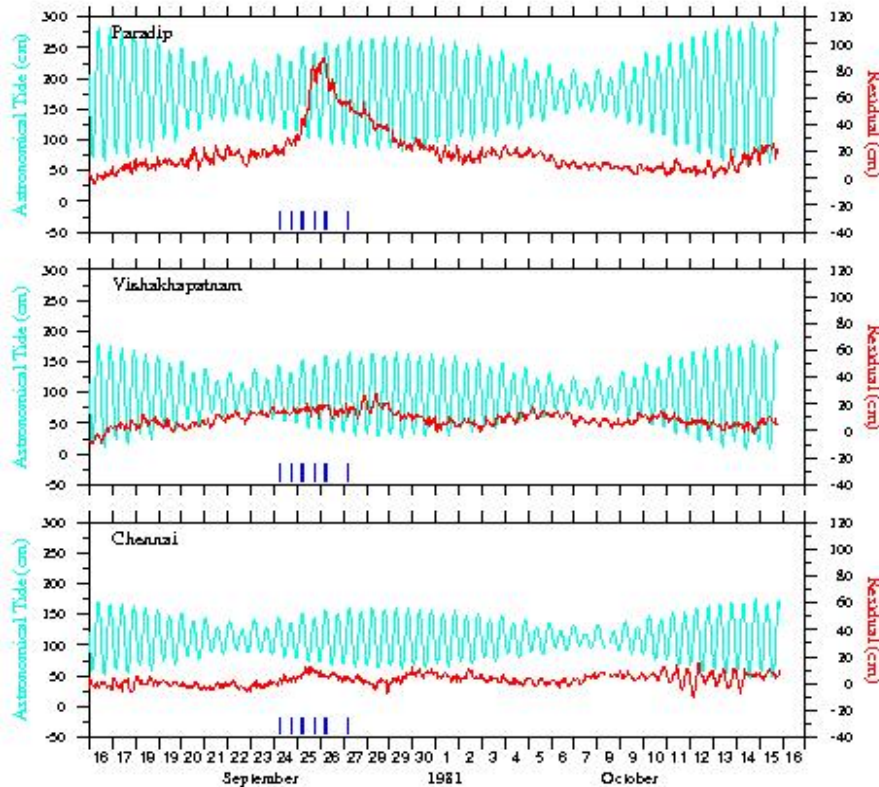
Figure 3 b. As in Figure 1 ft, but for Event 3. The resulting surge was the largest, as in Event 2, at Paradip. In contrast, however, the peak surge occurred at the time of high tide. In addition, the tide at this time was mid-way between the neap and the spring tide. As a result, the water level during this event was much higher than that in Event 2, even though the storm-related surges in sea level in the two events were of similar magnitude. Had the storm surge occurred about 6 h later, at the time of low tide, the net water level would have been almost 1.5 m lower than what was actually experienced. That the difference of a few hours in the timing of the peak can make considerable difference in the resulting damage underlines the difficulties that forecasters face in predicting sea level and issuing warning regarding the peak surge. This event was recorded only at Paradip; it did not have any significant impact on the sea-level at Visakhapatnam and Chennai.
