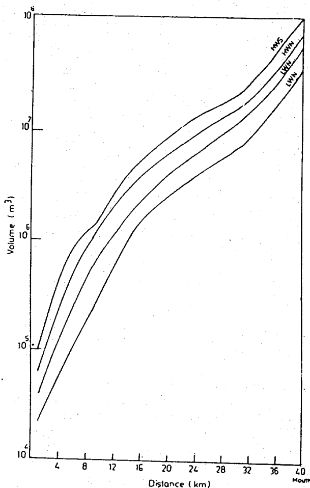
Fig. 2—Cumulative volume of estuary against distance (LWN—low water neap; LWS—low water spring; HWN—high water neap; HWS—high water spring)
