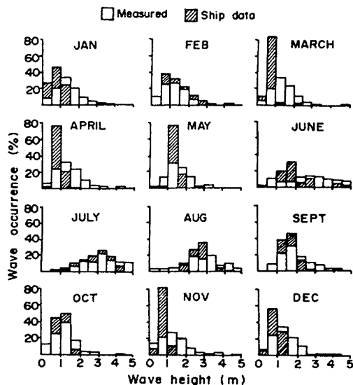
Fig. 3—Comparison of ship reported waves of grid 9 and the measured waves at Bombay High
