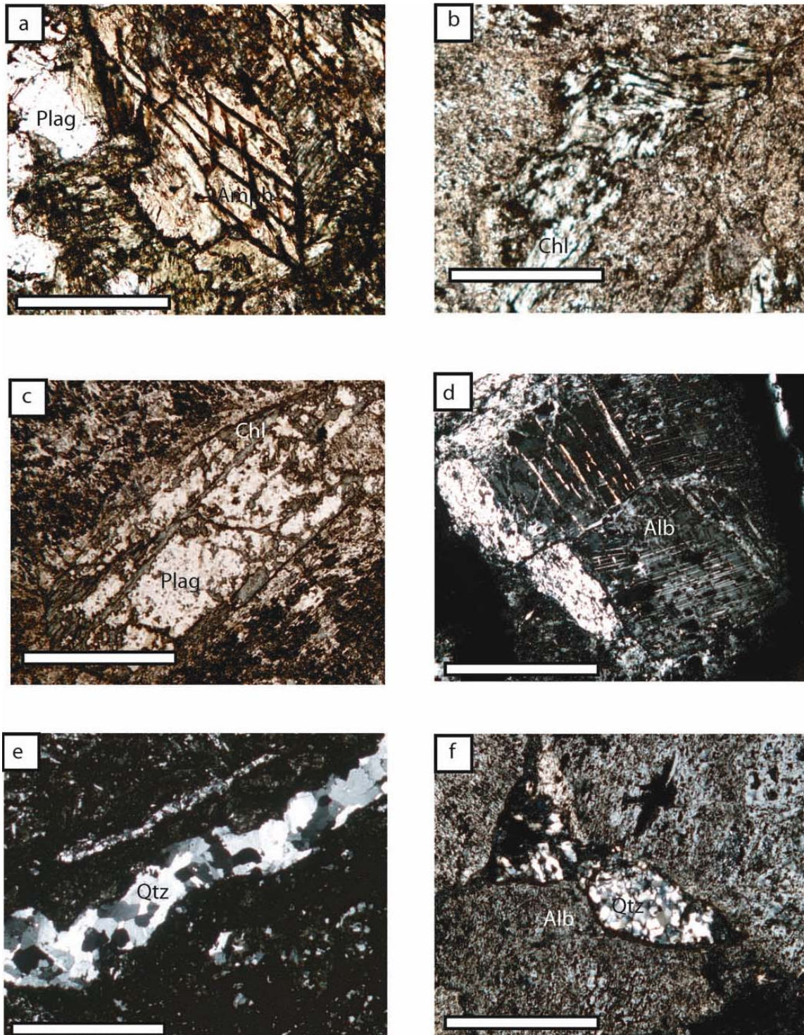
Figure 3. Photomicrographs of altered gabbro from corner-high (station DR 02). (a) Magnesio hornblende (Amph) with prominent cleavage trace (PPL \times 10X). (b) Deformed chlorite (Chl) band within albitised matrix (PPL \times 5X). (c) Chloritisation of plagioclase along fractures formed within the plagioclase phenocryst (PPL \times 5X). (d) Twinning within albite (Alb). (XPL \times 10X). (e) Late quartz vein (Qtz). (XPL \times 5X). (f) Recrystallised Qtz grains enclosed by albite (Alb) phenocrysts (XPL \times 5X). Scale bar: 0.5 mm for figure 2(a, d) and 1 mm for figure 2(b, c, e, f).
