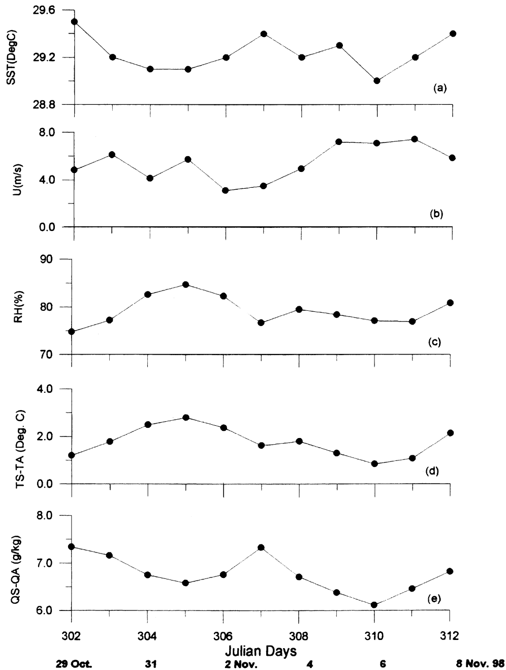
Figure 9. Along the track daily variation of (a) sea surface temperature, (b) wind speed, (c) relative humidity, (d) sea minus air temperature at 10 m height above the surface and (e) sea minus air specific humidity difference at 10 m height above surface during BOBMEX-Pilot.
