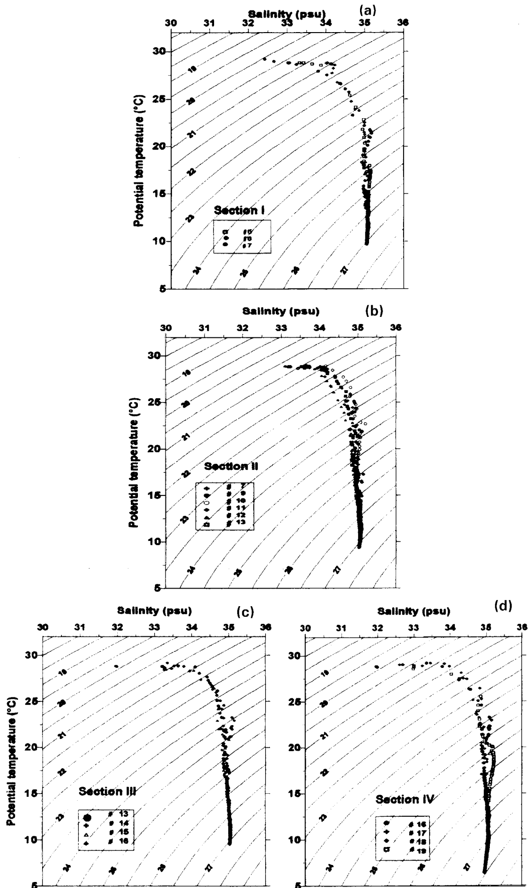
Figure 5. Watermass structure at the CTD stations along section I (a), section II (b), section III (c) and section IV (d) during BOBMEX-Pilot.
