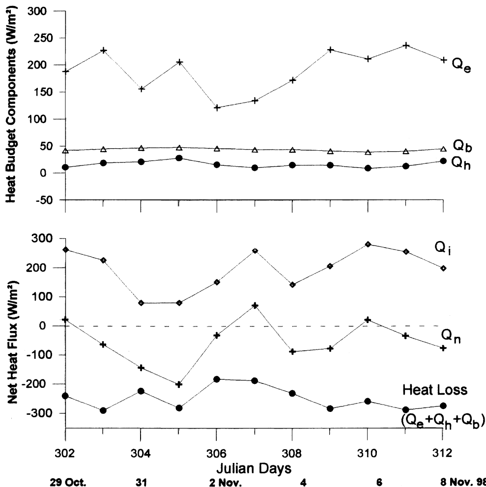
Figure 10. Along track daily variation of (a) heat budget components ( Q_e , Q_h , and Q_b ) and (b) net surface heat flux ( Q_n ). Incoming solar radiation ( Q_i ) and total heat loss ( Q_e + Q_h + Q_b ) during BOBMEX-Pilot.
