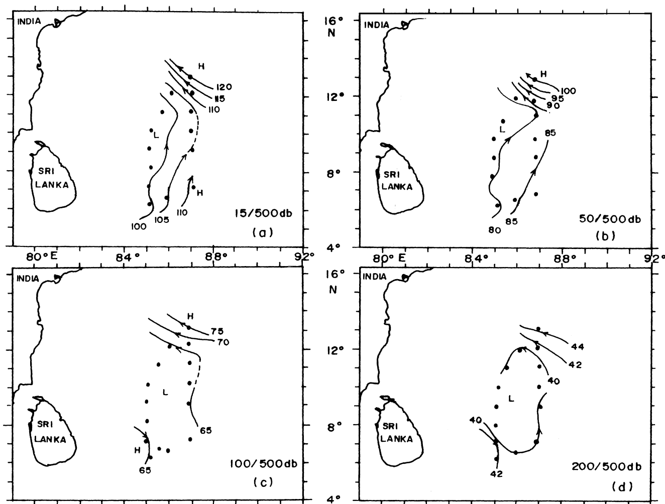
Figure 6. Dynamic topography (dyn.cm) maps relative to 500 db at various depths: (a) sea surface, (b) 50 m, (c) 100 m and (d) 200 m, during BOBMEX-Pilot.
