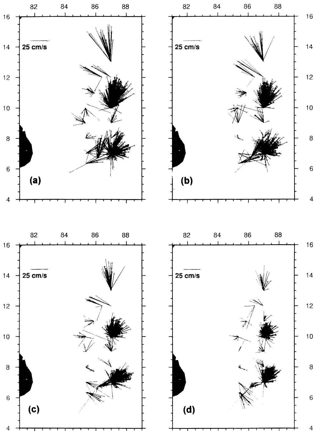
Figure 8. VM-ADCP measured ocean current vectors at the CTD stations at various depths: (a) 31 m, (b) 51 m, (c) 100 m and (d) 200 m during BOBMEX-Pilot. Note the cluster of vectors at 7^{\circ}\text{N} , 10^{\circ}\text{N} and 13^{\circ}\text{N} represent the time-series observations over a period of 48 hr, 48 hr and 24 hr respectively.
