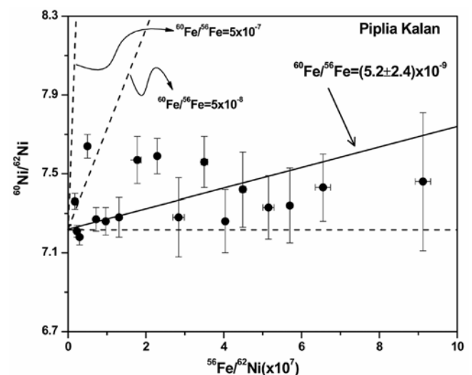
Figure 2. Fe–Ni isotope plot for Piplia Kalan. The inferred initial ^{60}\text{Fe}/^{56}\text{Fe} is 2\sigma . The error bars plotted are 1\sigma to have clarity. The result is based on least square fit using provost (1990). The horizontal dashed line is for normal terrestrial value. Correlation lines were forced to pass through the normal ^{60}\text{Ni}/^{62}\text{Ni} value. The other two dashed lines for initial ^{60}\text{Fe}/^{56}\text{Fe} of 5 \times 10^{-7} and 5 \times 10^{-8} respectively, are shown for comparison.
