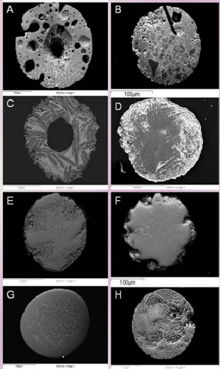
Figure 2. Polished sections of cosmic spherules from the Indian Ocean : A – F are S-type cosmic spherules in the sequence of increasing melting and evaporation as classified by Taylor et al. (2000).
