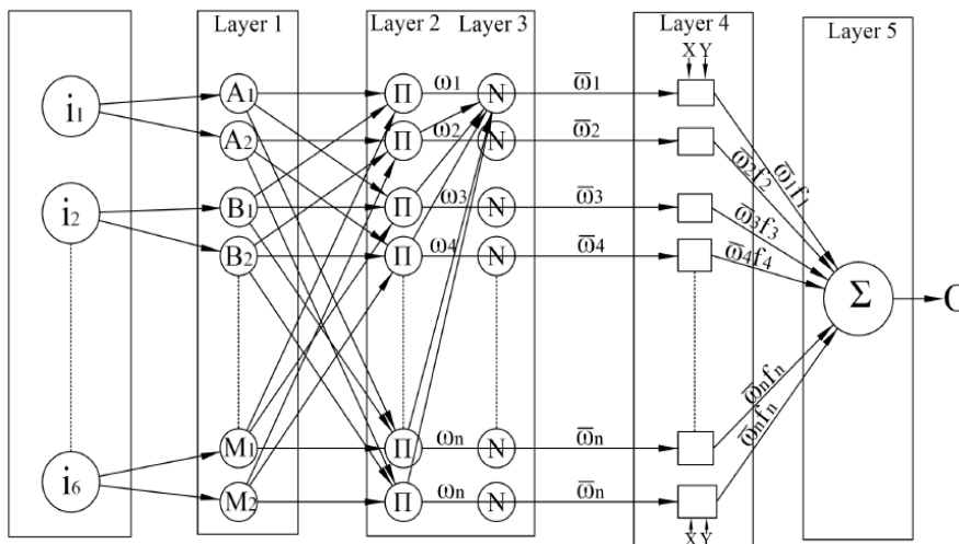
Fig. 4 ANFIS structure.
