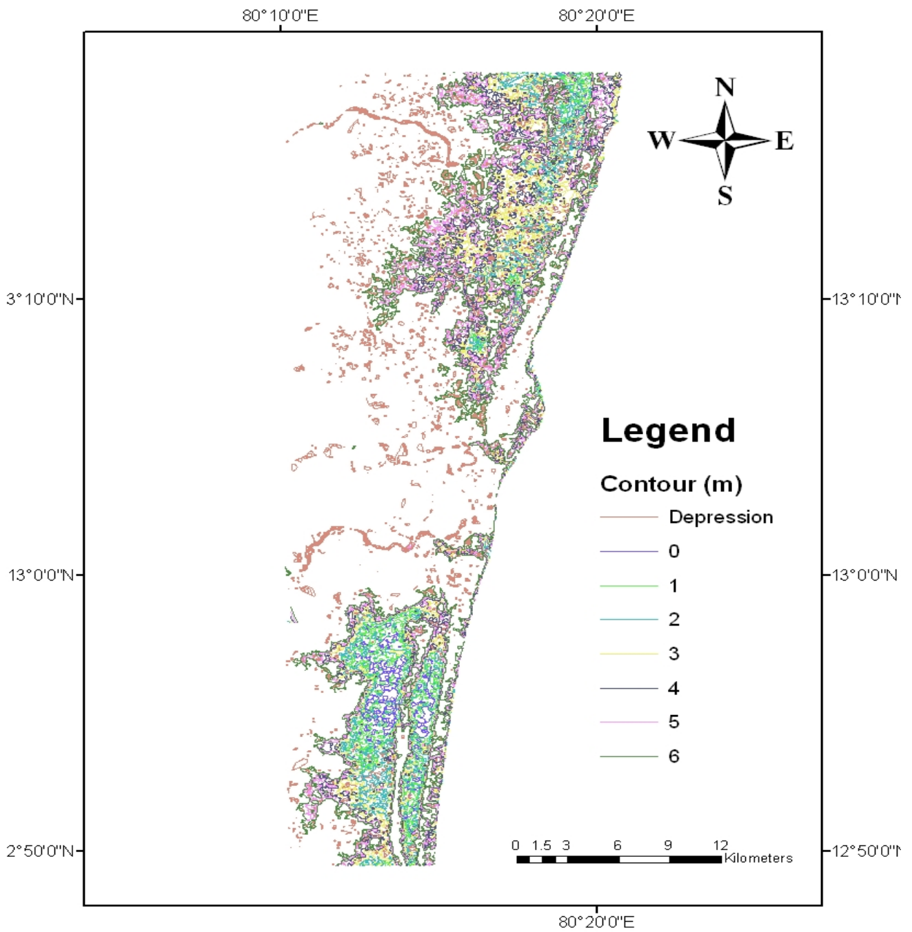
Fig. 5 Contour Map developed from SRTM Data Showing Coastline and Rivers
