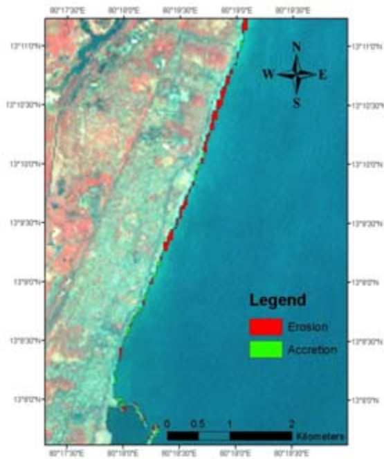
Fig. 2c Chennai – Section 3 showing Accretion and Erosion
