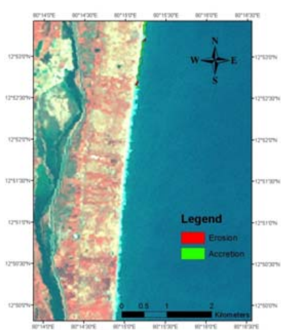
Fig. 2h Chennai – Section 8 showing Accretion and Erosion
