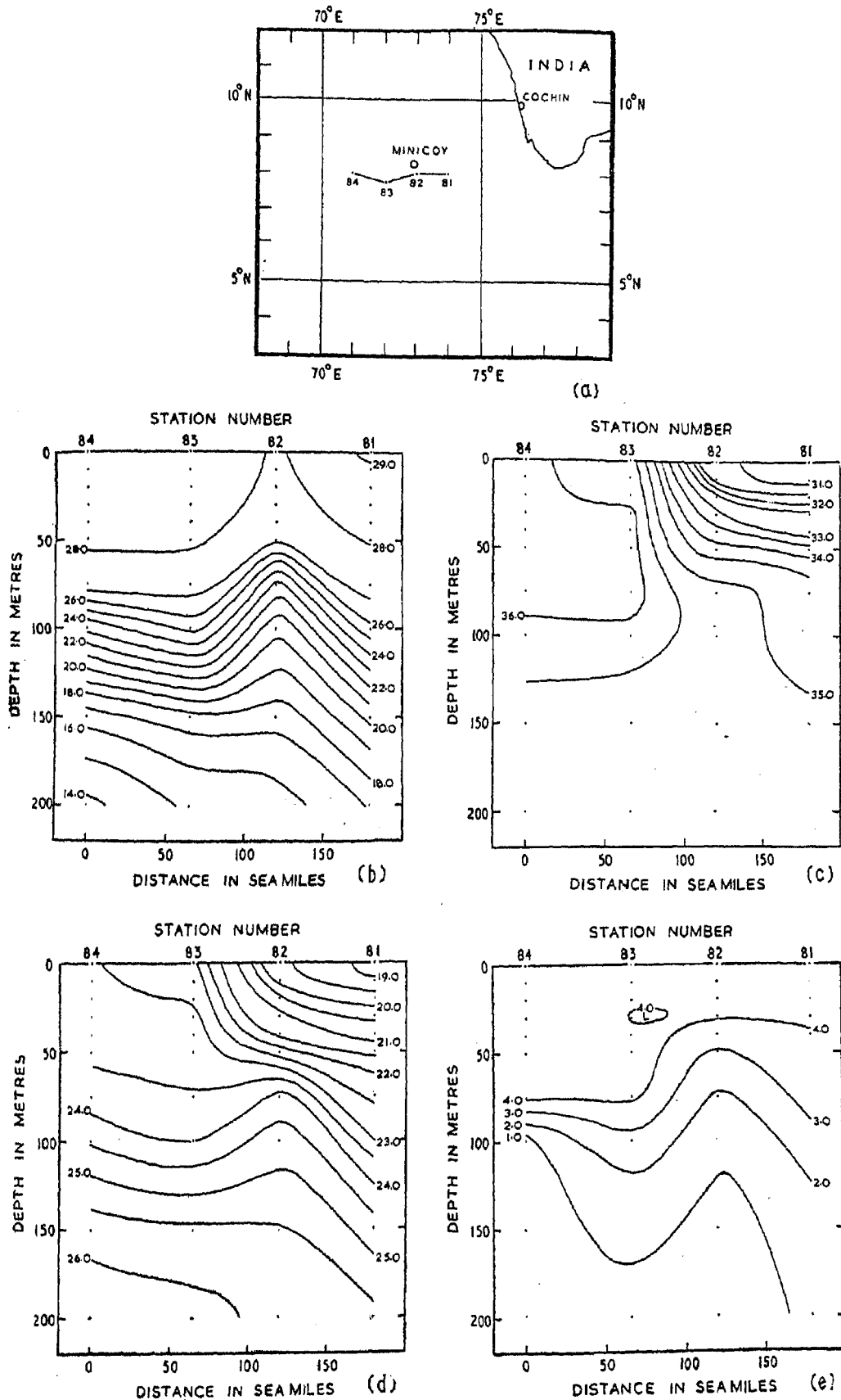
FIG 1 Vertical distribution of temperature, salinity, density and dissolved oxygen along a section south of Minicoy Island during the last week of November, 1962: (a) Shows the location of station along the section, (b) Shows the temperature distribution-contour interval 1 C. (c) Shows the salinity distribution-contour interval 0.5‰. (d) Shows the distribution of density in terms of \sigma_t contour interval 0.5 gm./litre. e) Shows the distribution of dissolved oxygen contour interval 1 ml/l.
