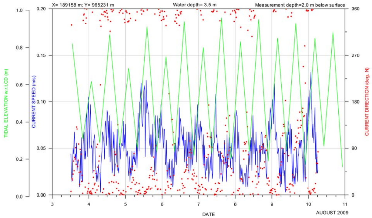
Figure 2. Variation of current speed and direction
