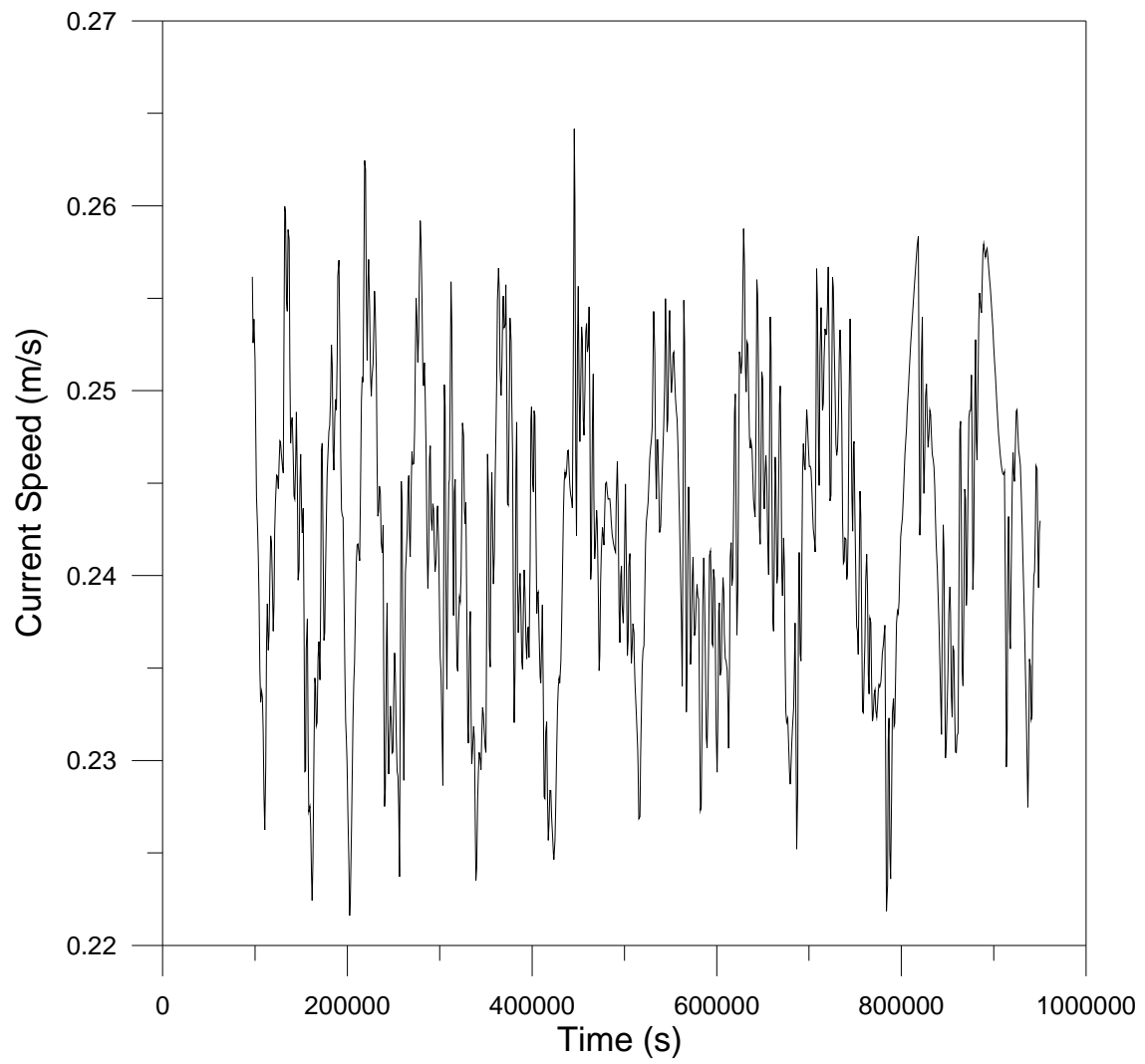
Figure 6. Temporal variations of currents during south west monsoon
