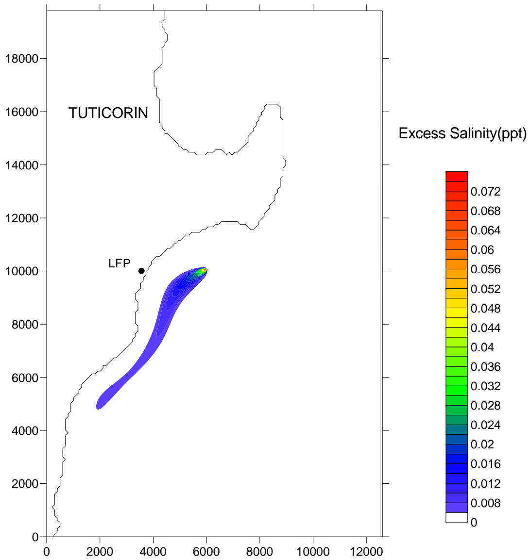
Figure 7. Modelled salinity during north east monsoon
