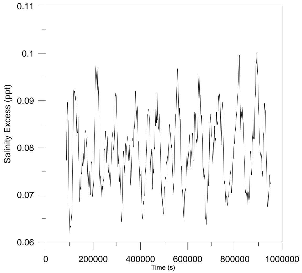
Figure 9. Temporal variations of salinity during north east monsoon
