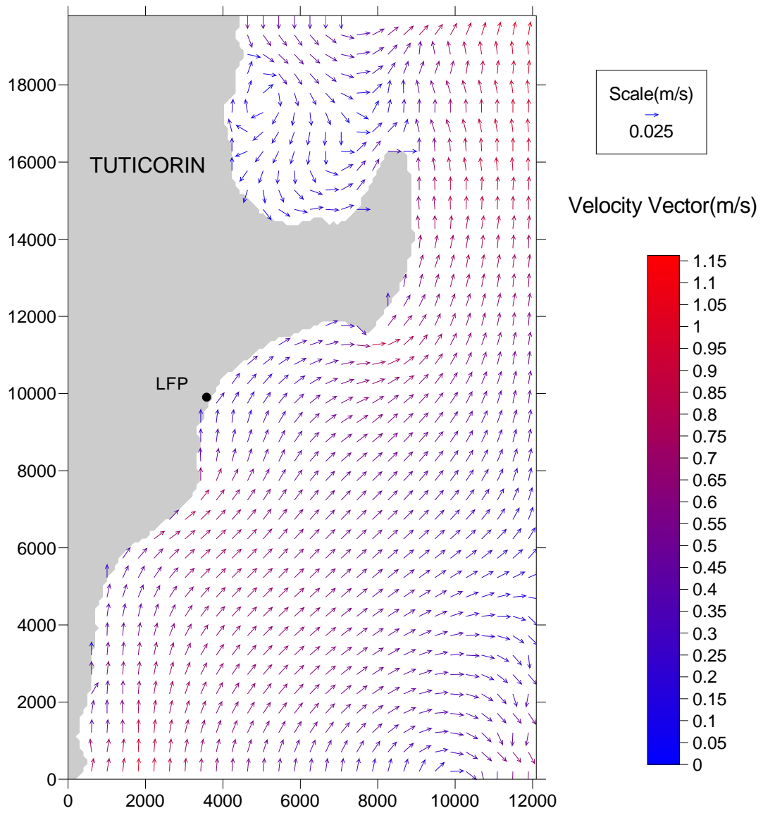
Figure 4. Modelled current during south west monsoon
