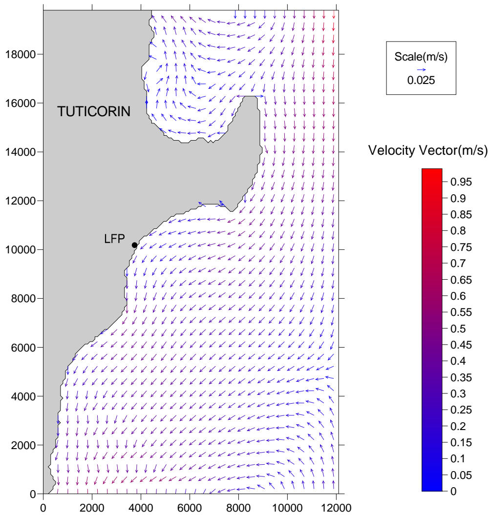
Figure 3. Modelled current during north east monsoon
