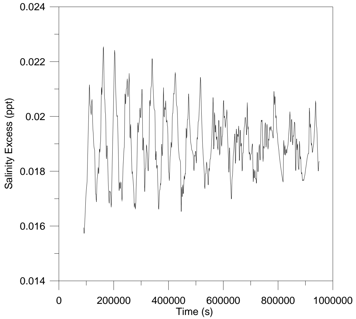
Figure 10. Temporal variation of salinity during south west monsoon
