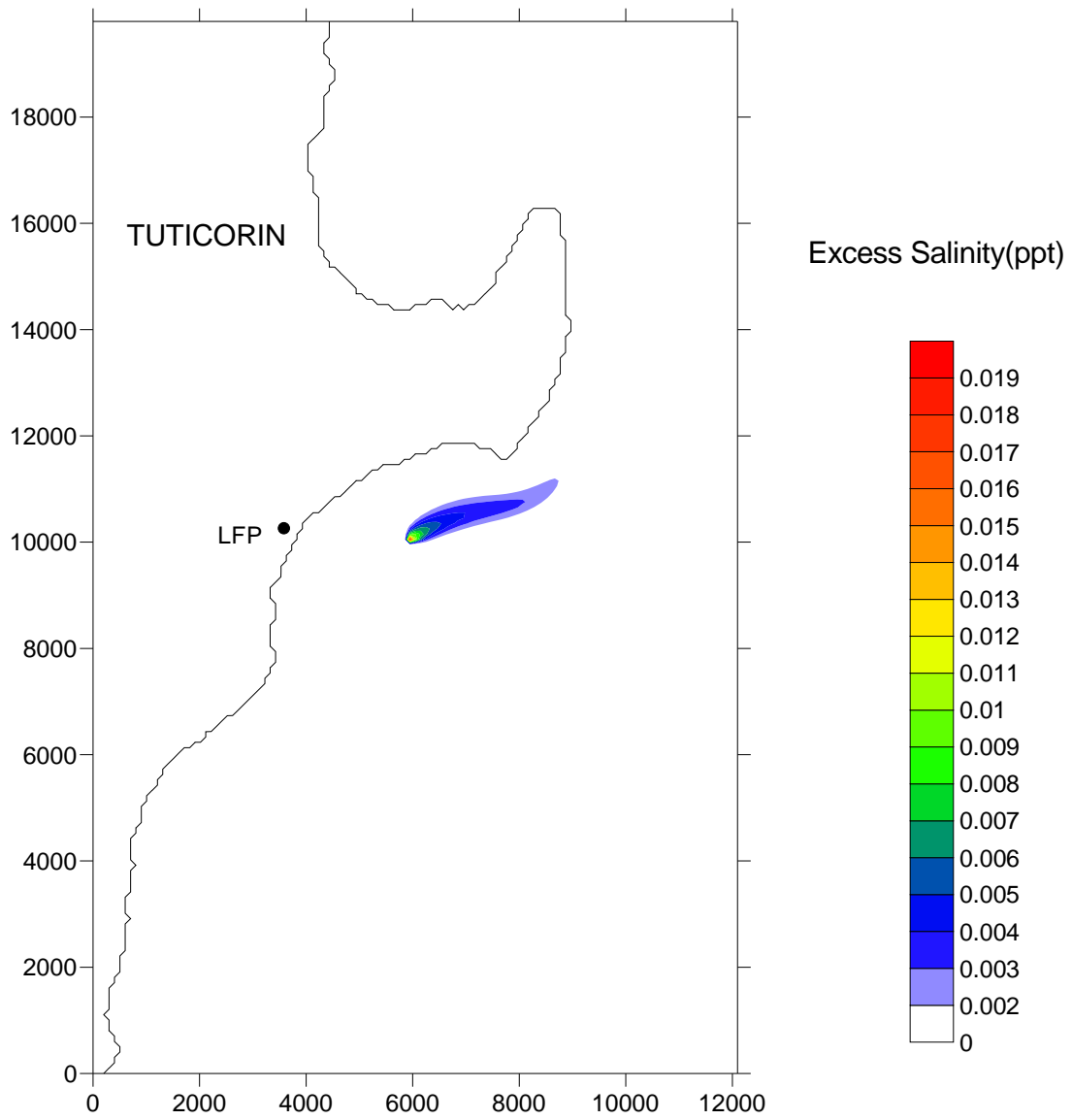
Figure 8. Salinity distribution during south west monsoon
