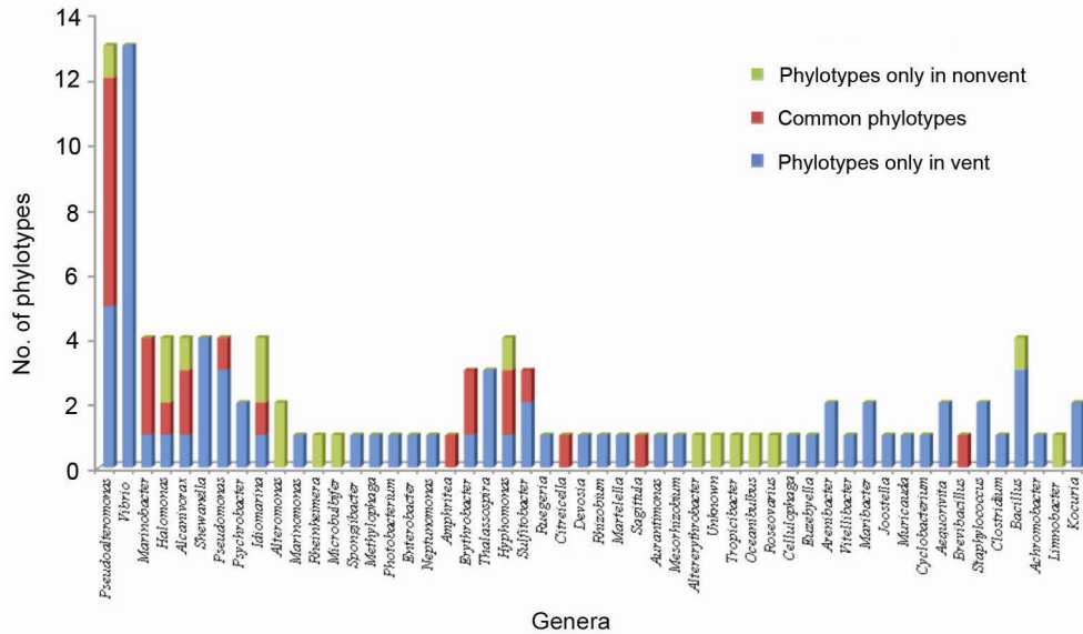
Figure 4. Number of vent, nonvent and common phylotypes retrieved from each genus.
