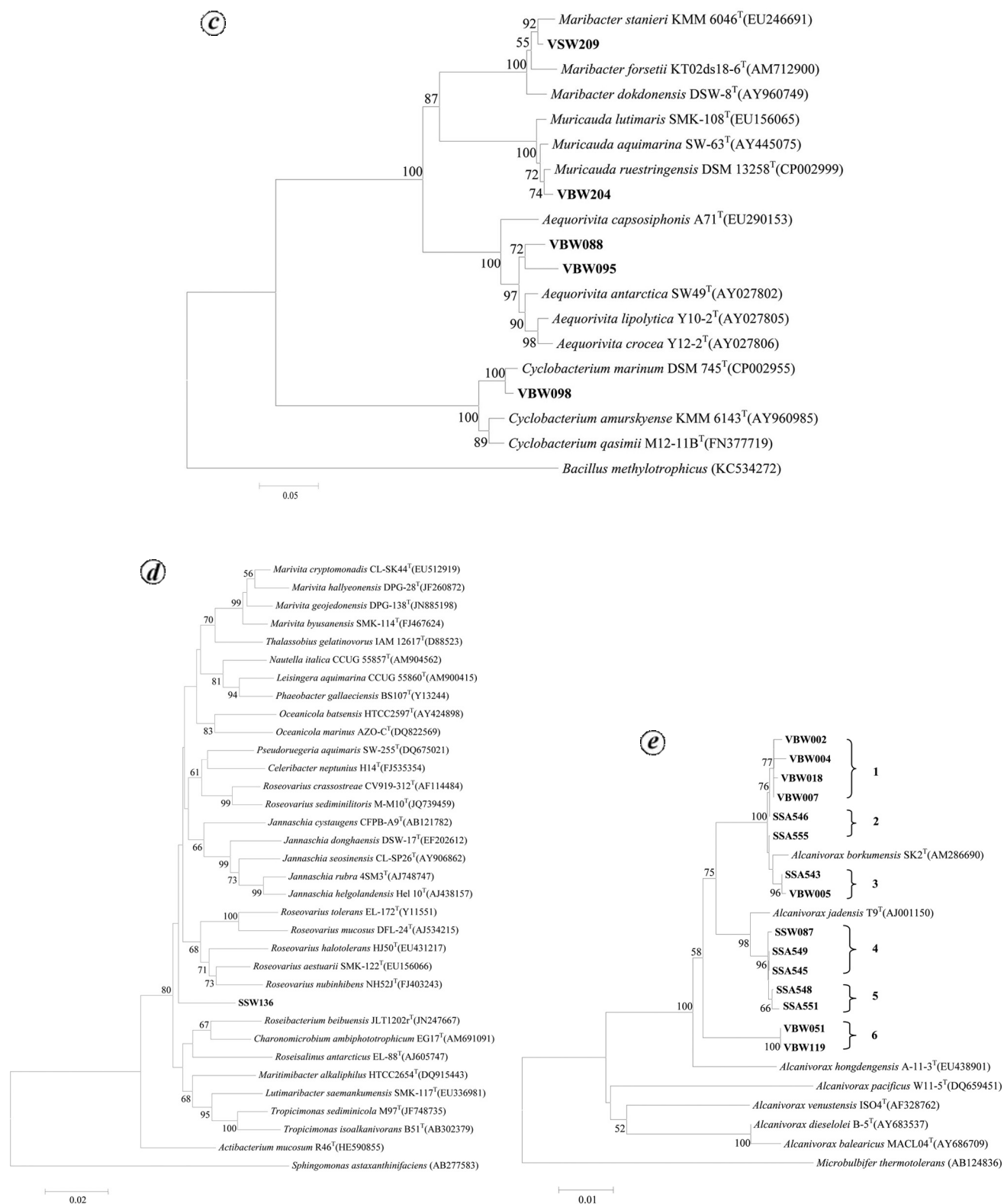
Figure 5. Phylogenetic relationships of representative novel taxa obtained from vent and nonvent regions of Espalamaca based on neighbour-joining analysis of 16S rRNA gene sequences data. The percentage of replicate trees in which the associated taxa clustered together in the bootstrap test (1000 replicates) is shown next to the branches. Bootstrap percentages of > 50 are shown on the nodes. The evolutionary distances were computed using the Maximum Composite Likelihood method. Bacillus methylotrophicus (KC534272) was used to assign an out-group for (a)–(d). Microbulbifer thermotolerans (AB124836) was used as out-group for (e). a–c, Phylogenetic relationships of novel species obtained from (a) \gamma -Proteobacteria; (b) \alpha -Proteobacteria and (c) Bacteroidetes. (d) Phylogenetic tree representing SSW136 as novel genus. (e) Phylogenetic variations of Alcanivorax isolates. Numbers from 1 to 6 indicate six possible groups of novel strains belong to the genus Alcanivorax .
