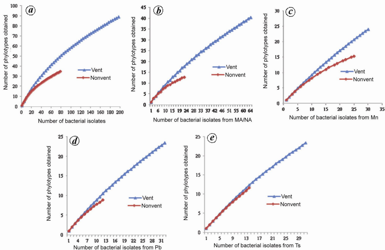
Figure 6. Rarefaction curves of operational taxonomic units (OTUs) based on 16S rRNA gene. Bacterial isolates were grouped into OTUs based at a level of sequence similarity of \geq 99\% . (a) Overall OTUs from vent and nonvent samples. b–e, OTUs from the isolation media: (b) Seawater nutrient agar (SWNA), (c) SWNA with 1 mM \text{MnCl}_2 , (d) SWNA with 1 mM \text{Pb}(\text{NO}_3)_2 and (e) SWNA with 0.5% thiosulphate.
