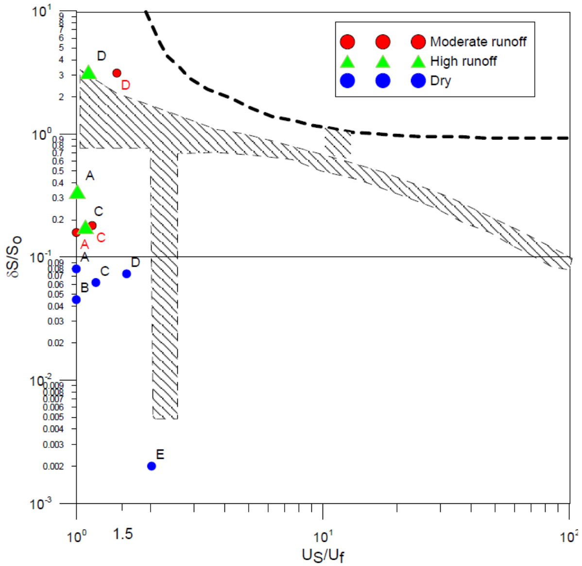
Fig. 6 Hansen –Rattray classification diagram for Cochin Estuary
