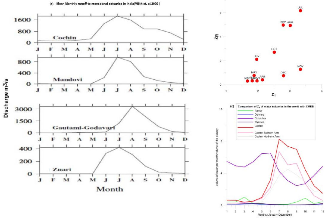
Fig. 7 Positions of each month of Cochin estuary on the ( Z_R , Z_T ) plane.
