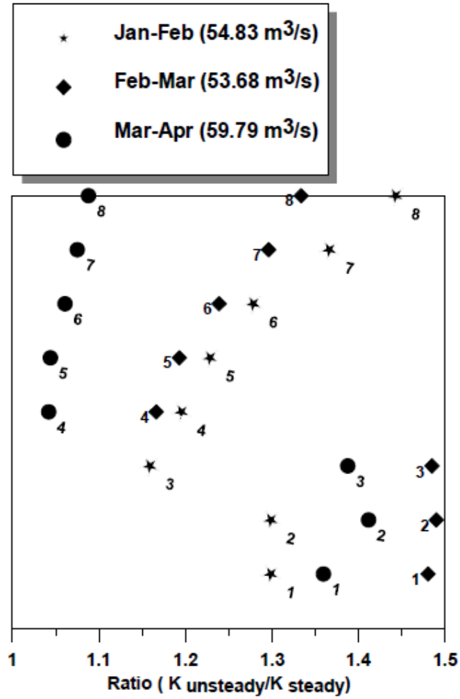
Fig. 8 The ratios of K_{\text{unsteady}} to K_{\text{steady}} calculated as shown in equation (7).
