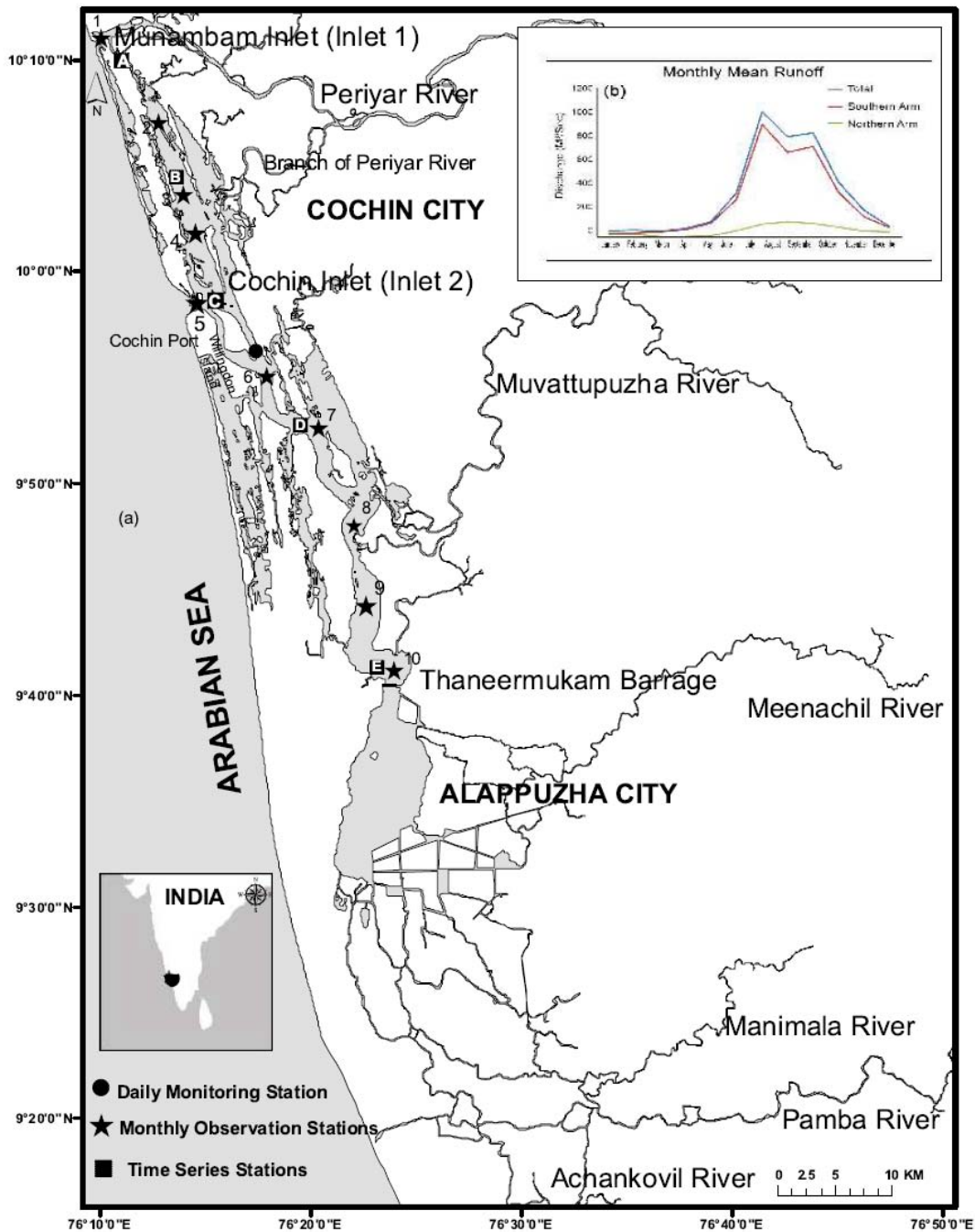
Fig. 1(a) The Cochin estuary (West coast, India), showing rivers and extent of the system, having two inlets to Arabian Sea, Munambam Inlet (north) and Cochin inlet (middle of the extent of the system). Daily station is located 5 km away from Cochin inlet. Monthly longitudinal and time series stations are discerningly marked. 1 (b) Runoff from 6 rivers for the period of 1 year (June 2008 to May 2009).
