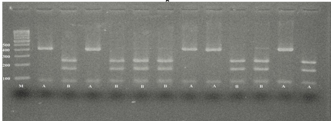
Figure 1 (a-d) shows the restriction digestion of mtDNA (D-loop) of Auxis spp. with enzyme Rsa I. Where M is the 100 bp DNA marker and A, B, C, D, E, F, G, H, I, and J are different haplotypes. (g-h) shows the restriction digestion of mtDNA (D-loop) of Auxis spp. with enzyme Hinf I. Where M is the 100 bp DNA marker and A, B, and C are different haplotypes.
