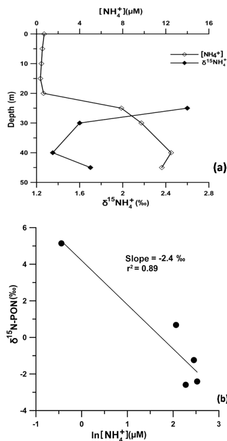
Figure 5. (a) Depth-wise variations of ammonium concentration and \delta^{15}\text{N-NH}_4^+ in May 2012. (b) Plot of \delta^{15}\text{N-PON} vs. \ln(\text{NH}_4^+) . The negative linear correlation yields a fractionation factor ( \epsilon ) of -2.4\text{‰} . Each data point represents a single sample.
