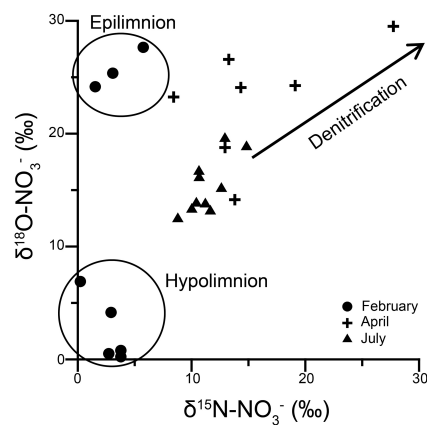
Figure 4. Nitrogen and oxygen isotopic composition of dissolved nitrate during three different periods in 2014. February represents the early or weak stratification period with two distinct clusters of epilimnetic (0–10 m) and hypolimnetic (15–48 m) samples. April is a period of intense water-column stratification and a denitrification signal is observed in the bottom waters. July is a period of monsoon holomixis when the water column has uniformly high nitrate values.
