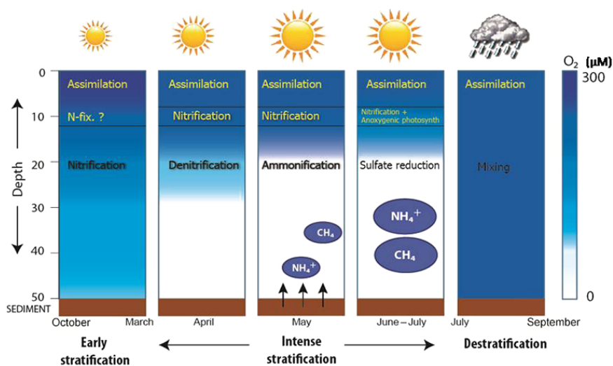
Figure 6. Schematic diagram depicting major biogeochemical processes taking place in the Tillari Reservoir over an annual cycle. This information is based on monthly sampling in the reservoir for several years (Shenoy et al., 2017).
