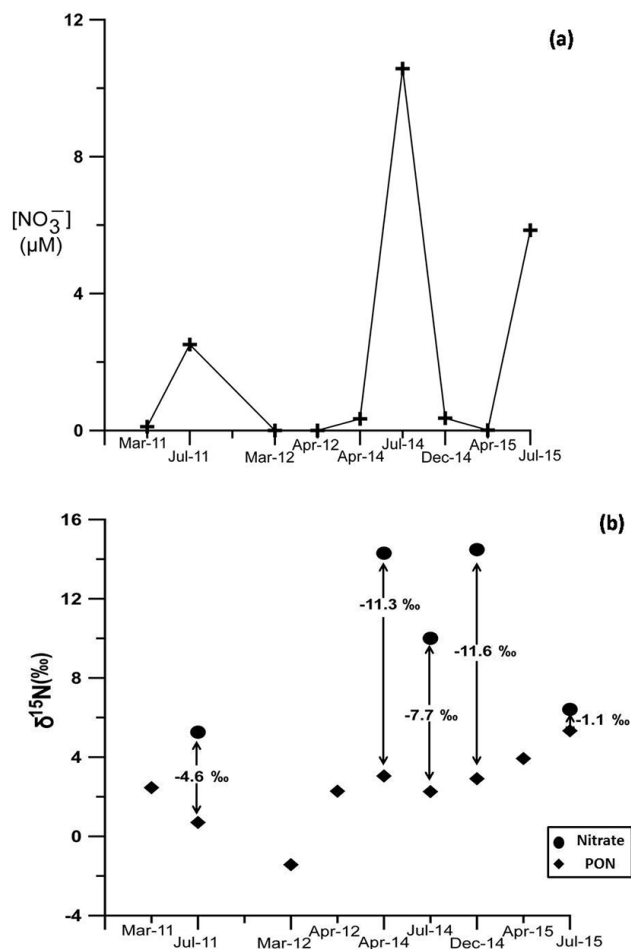
Figure 3. Time series of nitrate concentrations (a) and \delta^{15}\text{N} of dissolved nitrate and POM in the epilimnion (0–5 m) (b). The isotopic differences between the dissolved and particulate species are denoted by arrows. Each data point represents a single sample.
