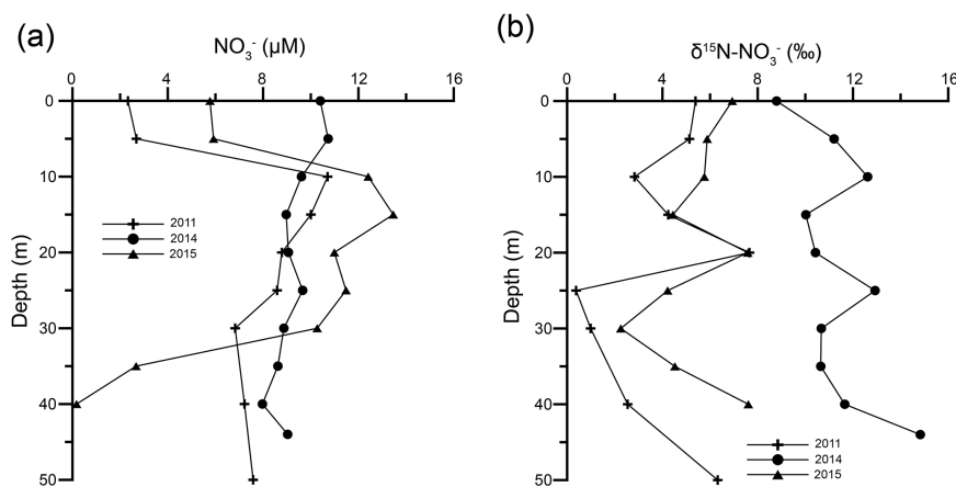
Figure 7. Vertical profiles of \text{NO}_3^- (a) and \delta^{15}\text{N-NO}_3^- (b) during monsoon mixing in 2011, 2014 and 2015. Each profile is from one field trip during the peak SWM in a given year with each data point representing one sample.
