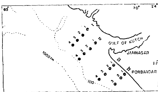
Fig. 2 — Station locations in the adjacent continental shelf
