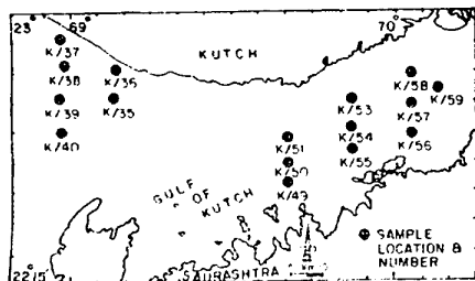
Fig. 1 — Station locations in the Gulf of Kutch
