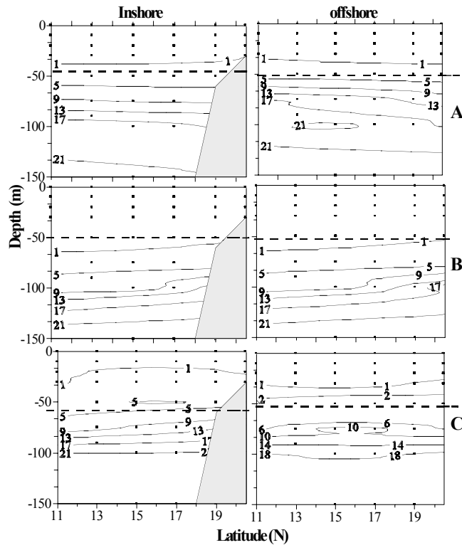
Figure 4. Vertical distribution of nitrate ( \mu\text{M l}^{-1} ) during (A) winter monsoon, (B) spring intermonsoon, and (C) summer monsoon.
