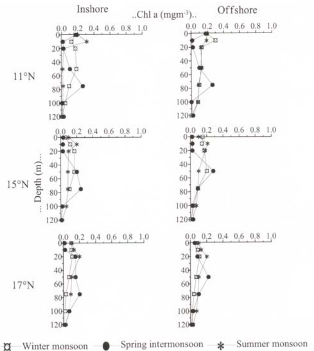
Figure 5. Seasonal trend in the vertical distribution of chlorophyll a (Chl a ).
