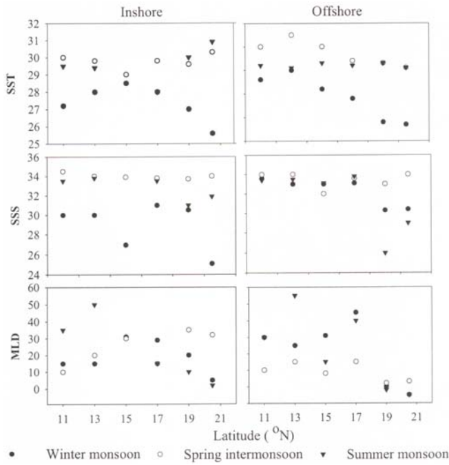
Figure 2. Seasonal and spatial variations of sea surface temperature (SST) ( ^{\circ}\text{C} ), sea surface salinity (SSS) (psu) and mixed layer depth (MLD) (m).
