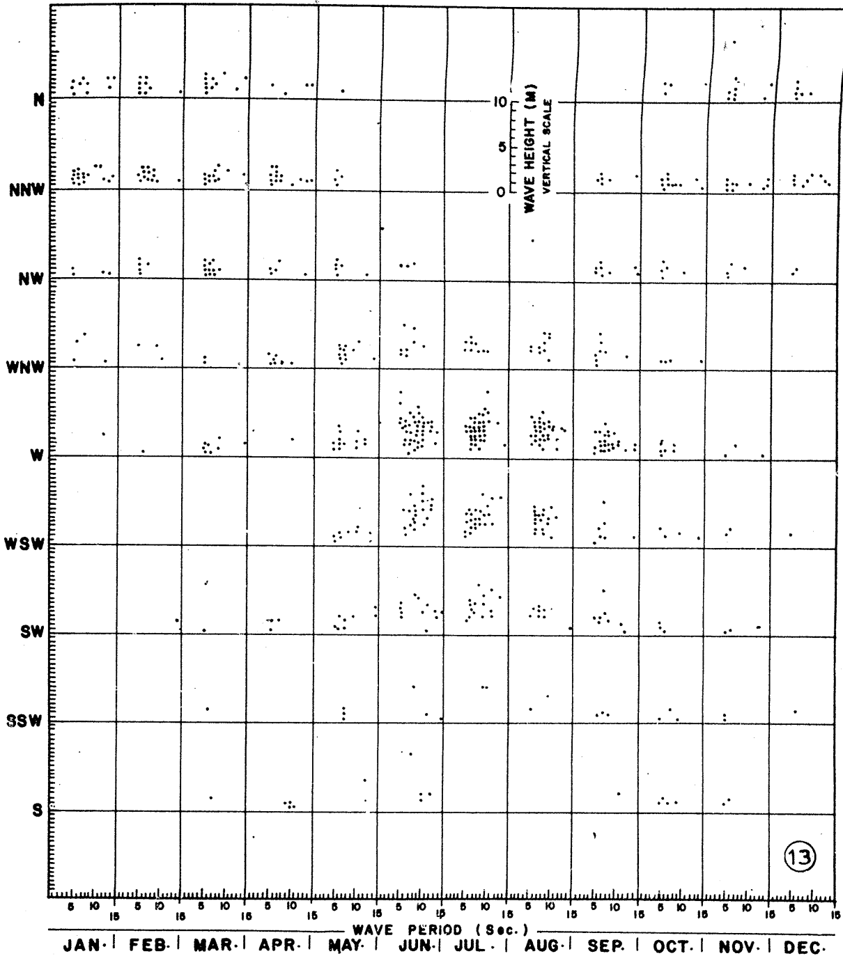
Fig. 13—Swell wave climate in the area 13°-18°N and 70°-74°E during 1970-'74
