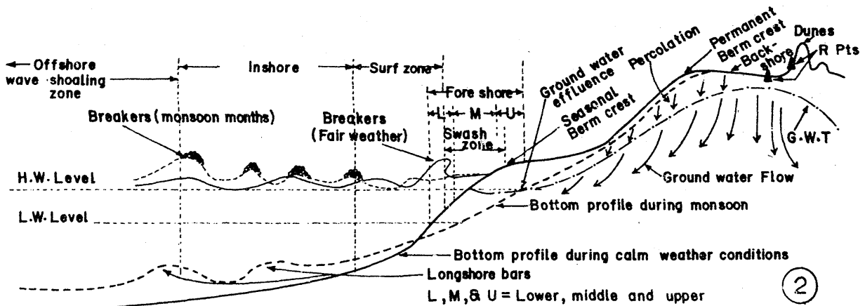
Fig. 2—Schematic picture showing the terminology of the beach adopted
