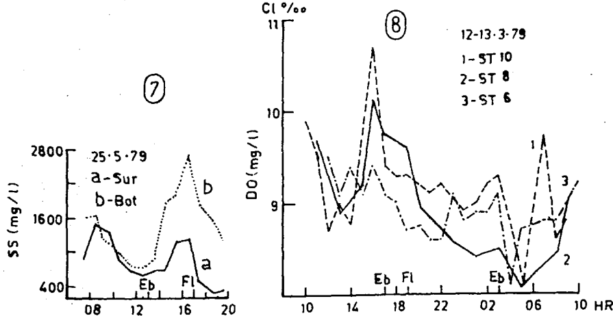
Fig. 7 - Variation of suspended solids with time at st 6
