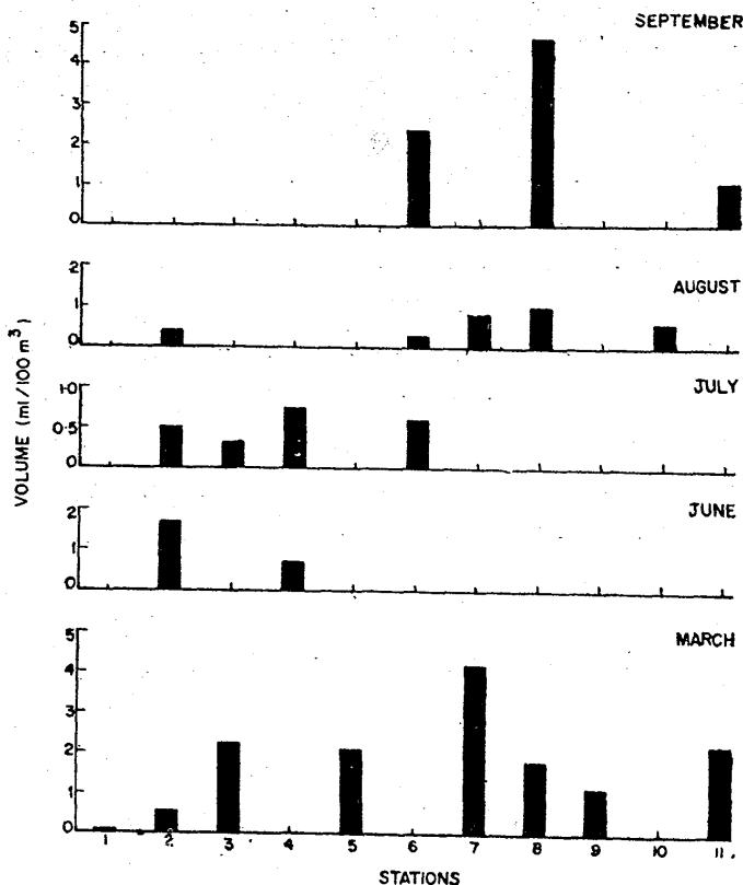
Fig. 3. Zooplankton biomass in the Narmada estuary during March to September 1979.
