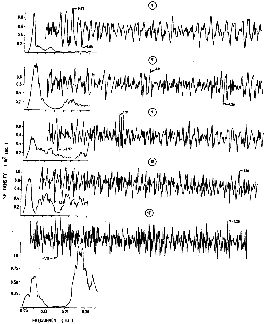
Fig. 1—Autospectra and corresponding surface wave profiles of selected wave records
