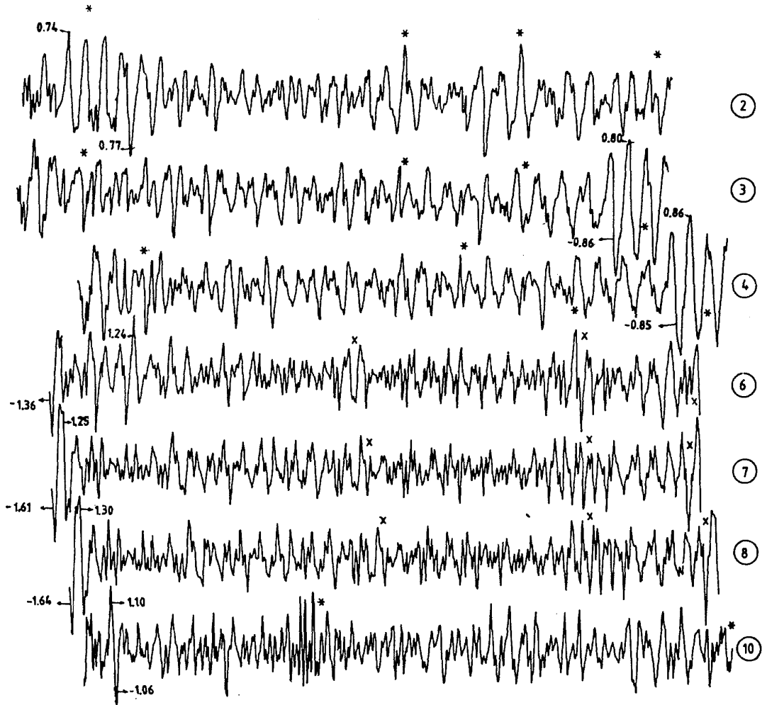
Fig. 2—Computed surface wave profiles with different ITUNE values [Profile numbers 2 to 4, 6 to 8 and 10 as in Table 1]
