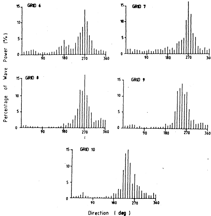
Figure 6. Directional distribution of wave power.
