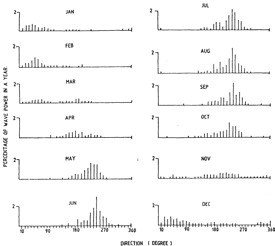
Figure 11. Percentage distribution of wave power in different directions during different months over a year.
