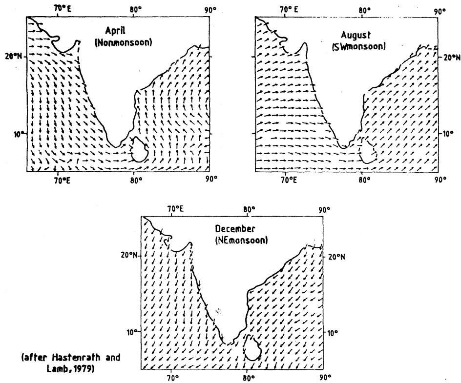
Figure 7. Seasonal wind pattern around Indian region.
