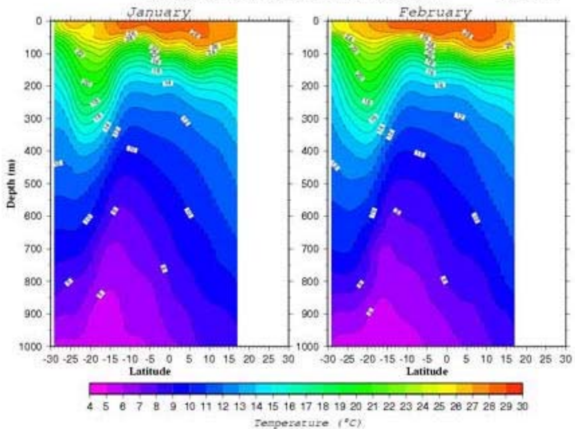
Temperature ( ^{\circ}\text{C} ) Section along 70.5^{\circ}\text{E}
