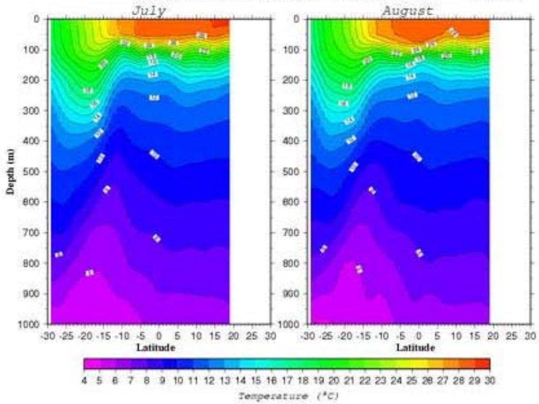
Temperature ( ^{\circ}\text{C} ) Section along 90.5^{\circ}\text{E}
