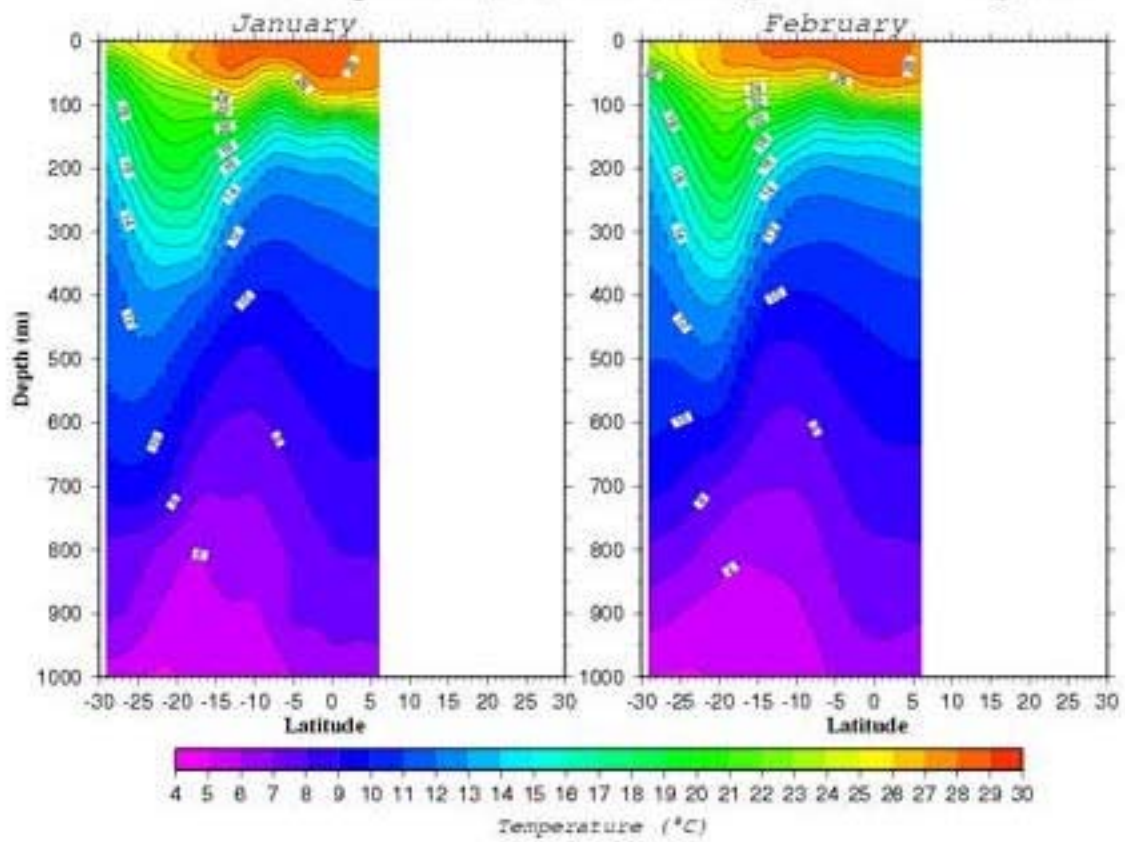
Temperature ( ^{\circ}\text{C} ) Section along 80.5^{\circ}\text{E}
