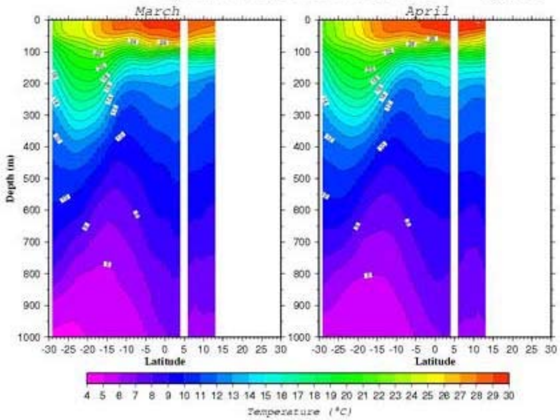
Temperature ( ^{\circ}\text{C} ) Section along 95.5^{\circ}\text{E}
