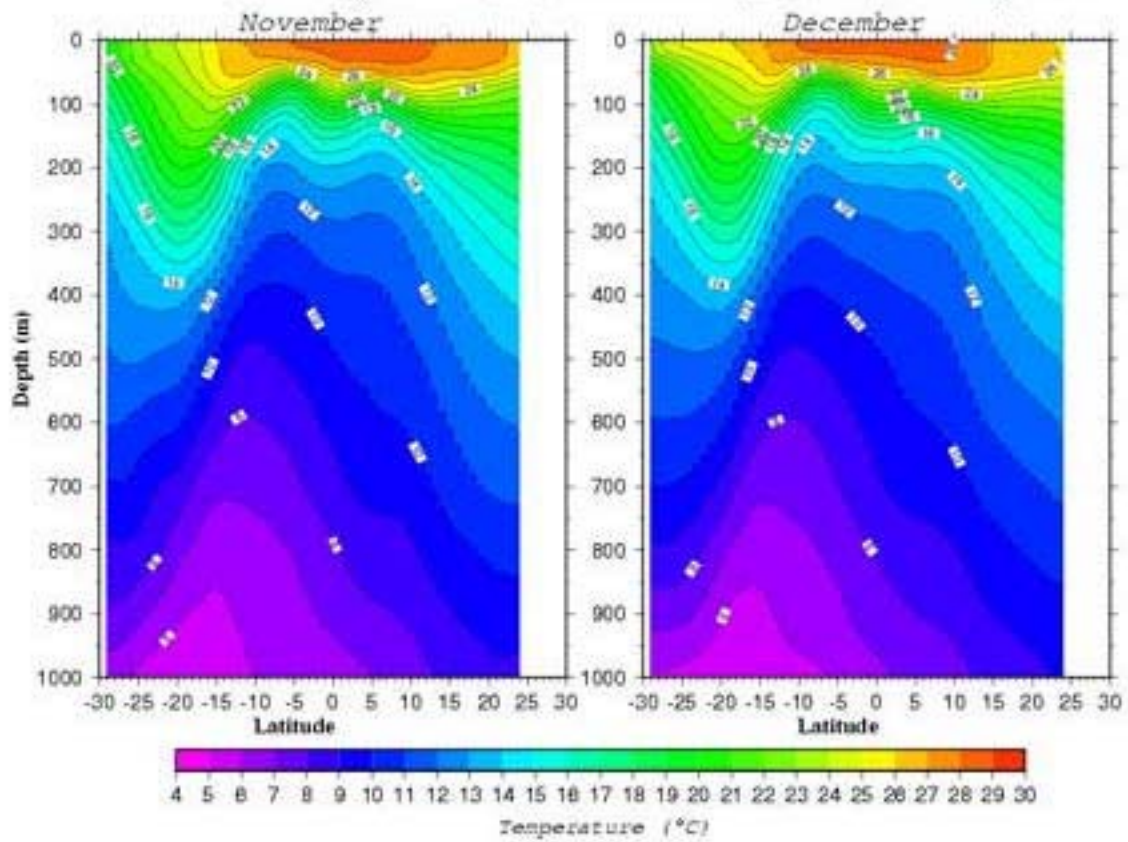
Temperature ( ^{\circ}\text{C} ) Section along 65.5^{\circ}\text{E}
