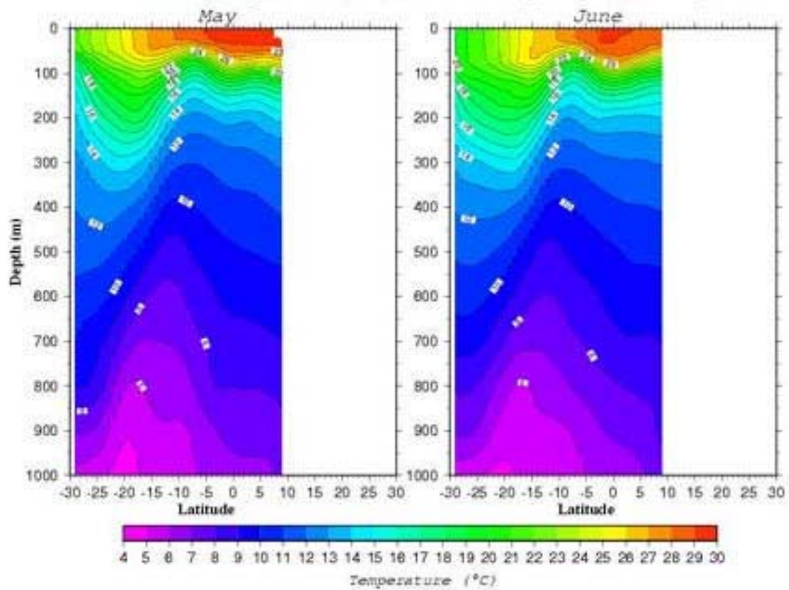
Temperature ( ^{\circ}\text{C} ) Section along 75.5^{\circ}\text{E}
