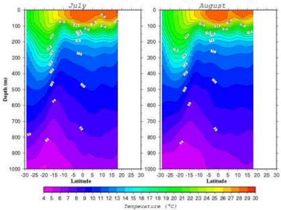
Temperature ( ^{\circ}\text{C} ) Section along 85.5^{\circ}\text{E}
