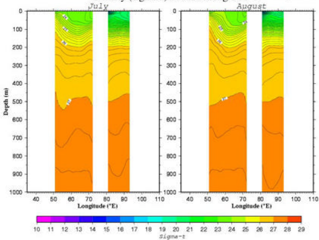
Density ( \sigma_t ) Section along 14.5°N Fig. B343
