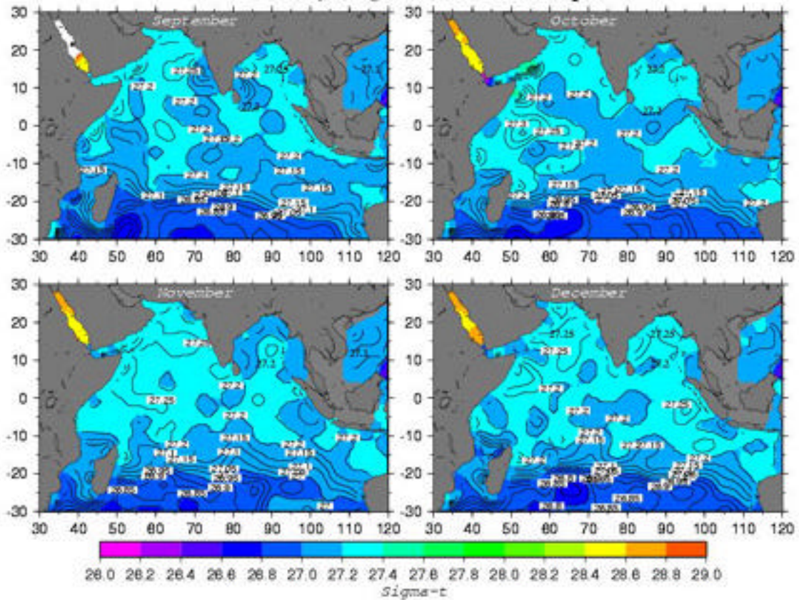
Density (Sigma-t) at 700 m depth
