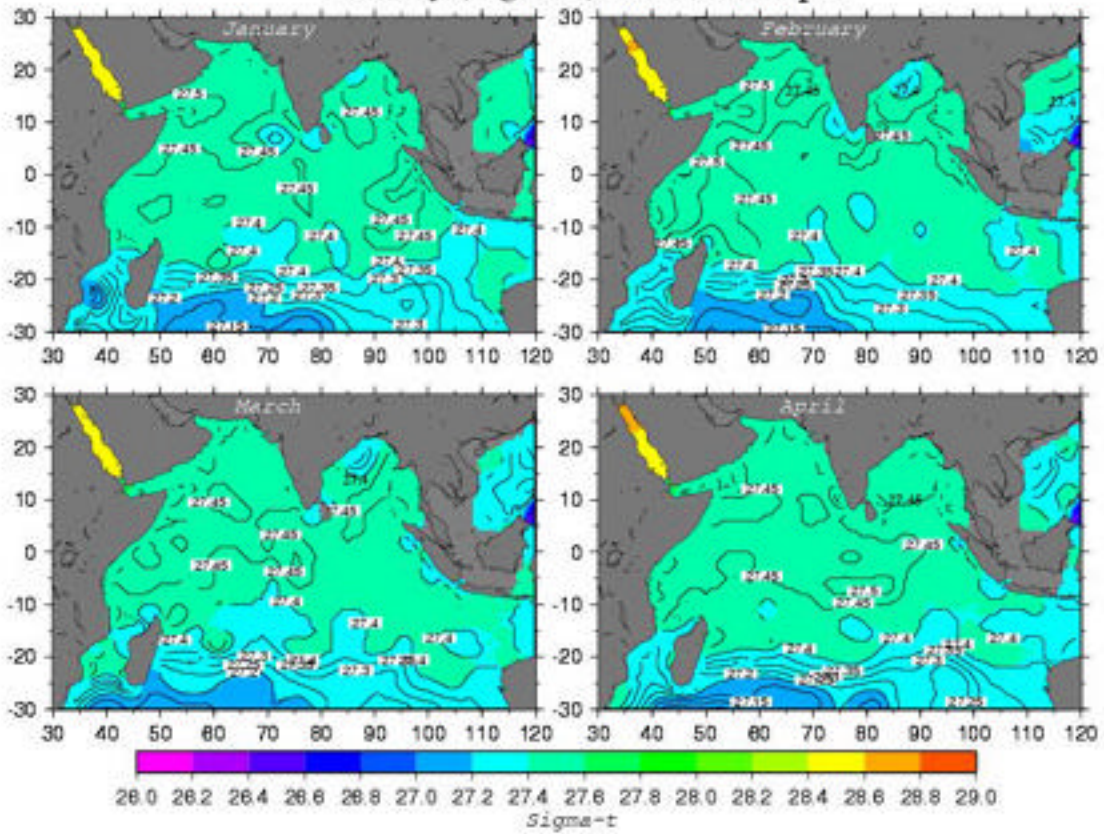
Density (Sigma-t) at 1000 m depth
