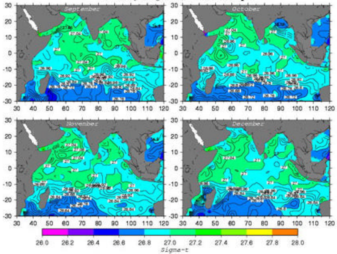
Density (Sigma-t) at 500 m depth
