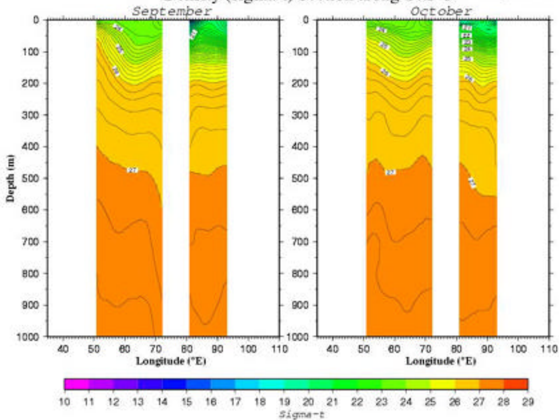
Density ( \sigma_t ) Section along 14.5°N Fig. B344
