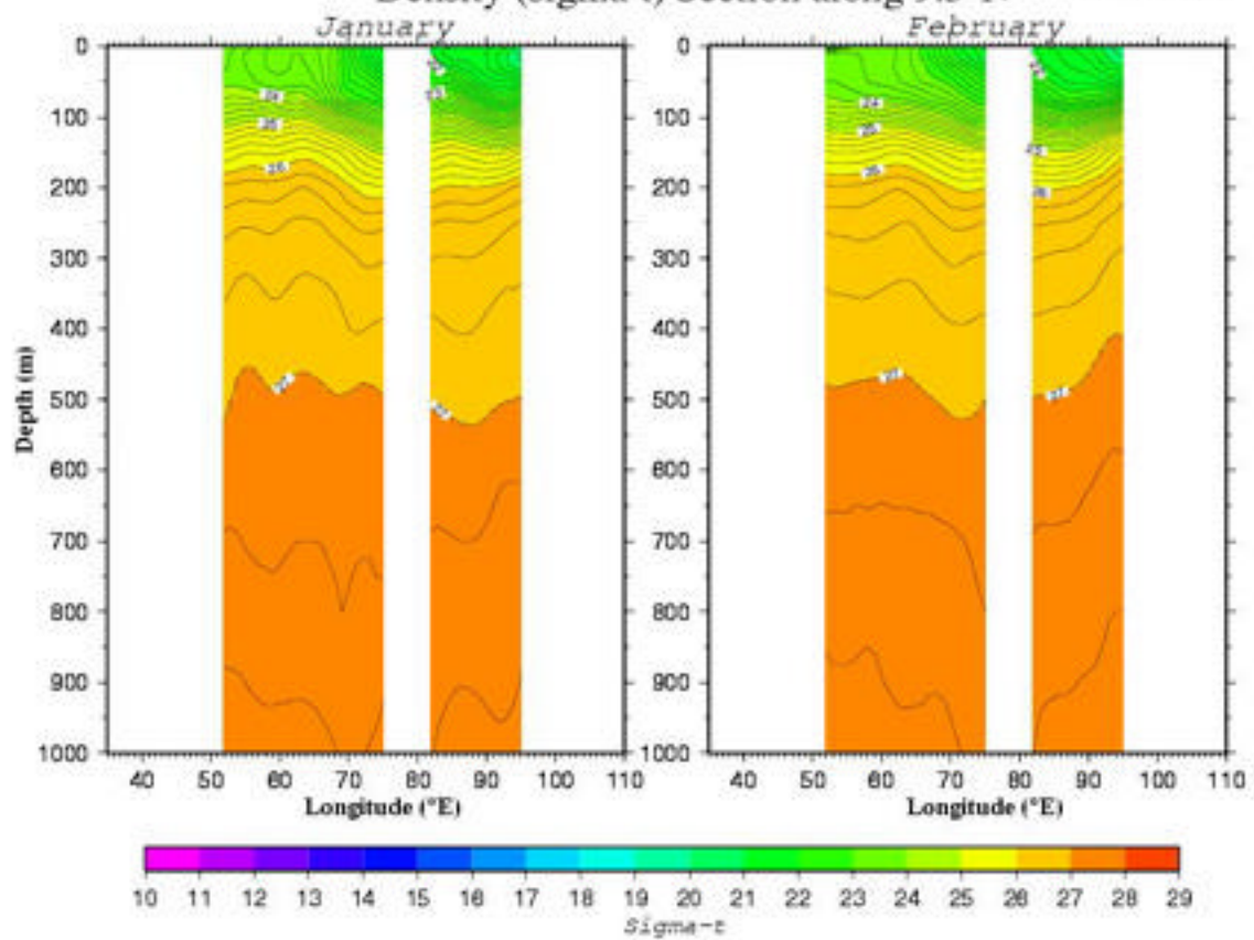
Density ( \sigma_t ) Section along 9.5°N Fig. B346
