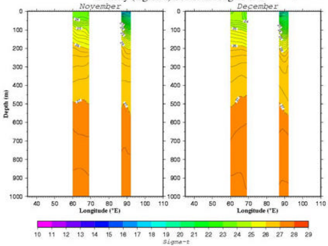
Density ( \sigma_t ) Section along 19.5°N Fig. B339
