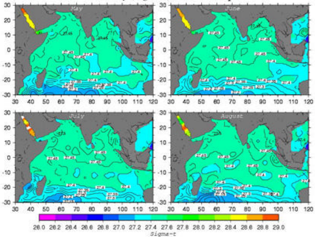
Density (Sigma-t) at 1000 m depth
