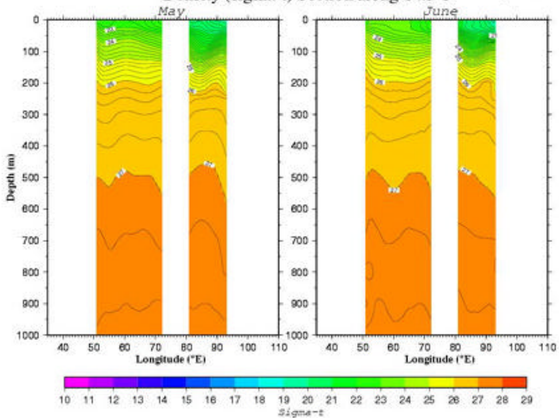
Density ( \sigma_t ) Section along 14.5°N
