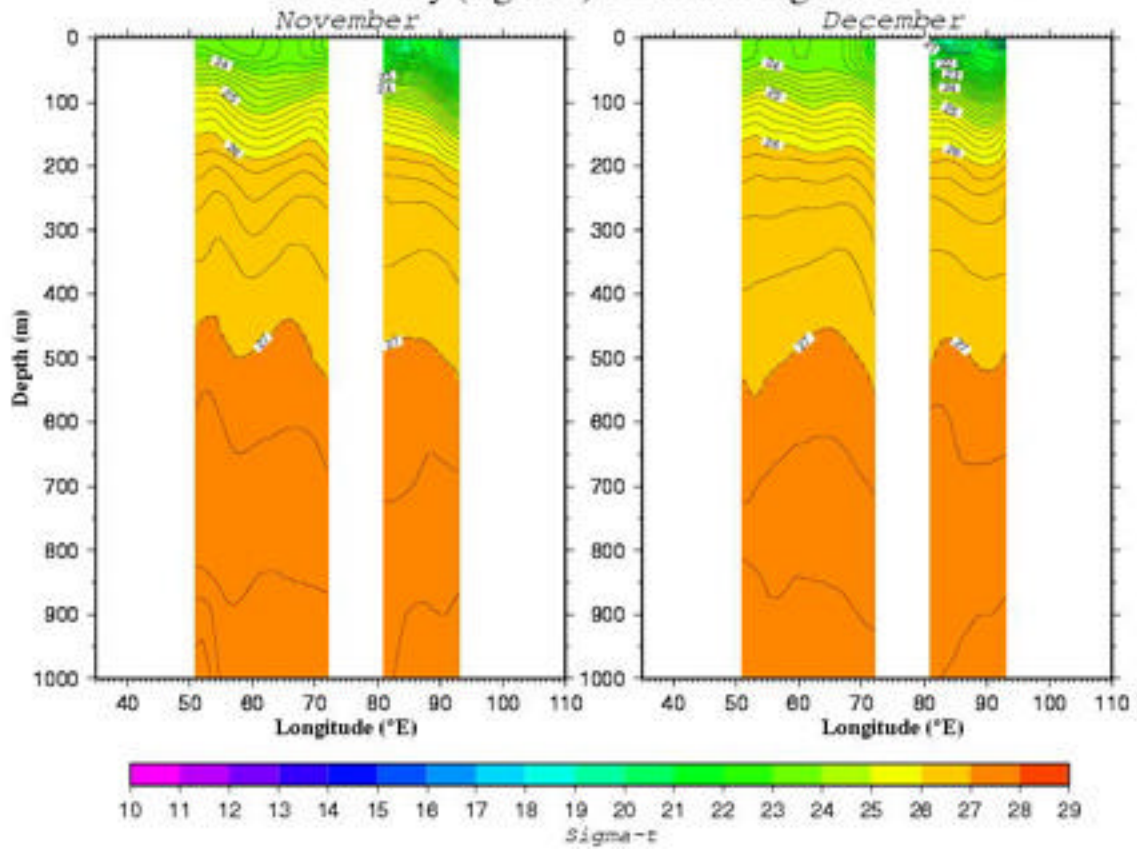
Density ( \sigma_t ) Section along 14.5°N Fig. B345
