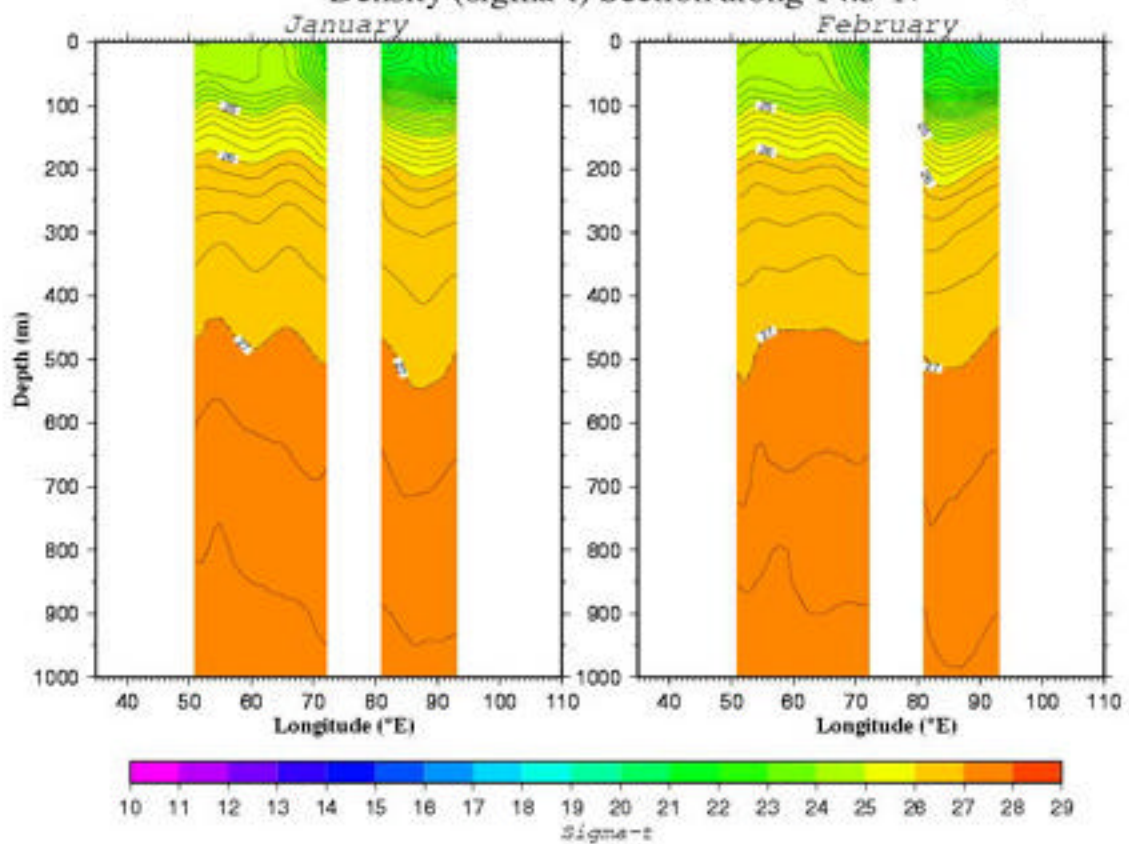
Density ( \sigma_t ) Section along 14.5°N Fig. B340
