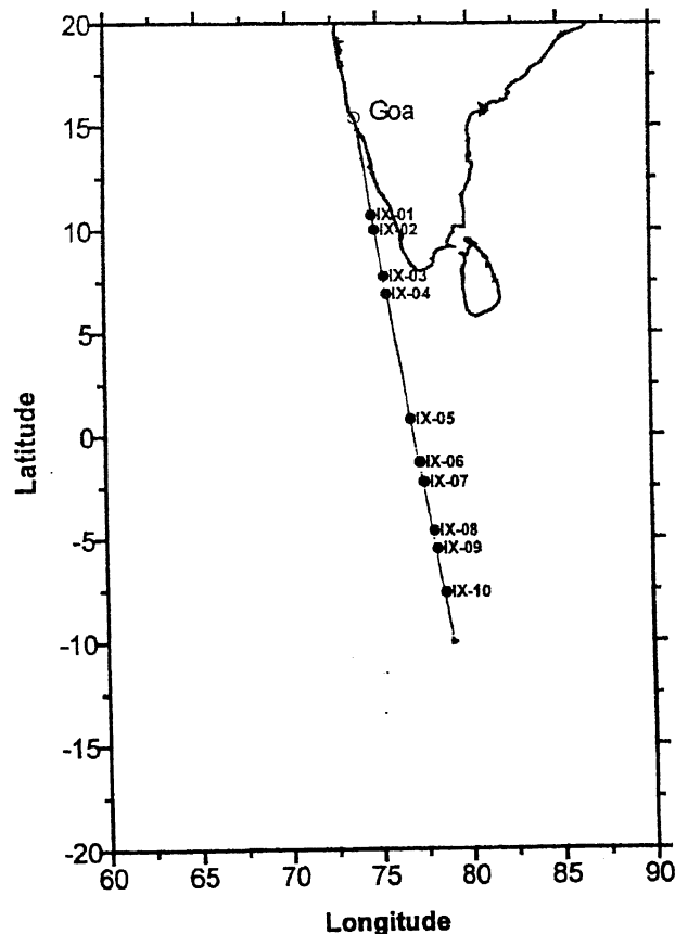
Figure 1. Location of conductivity–temperature–depth stations.
