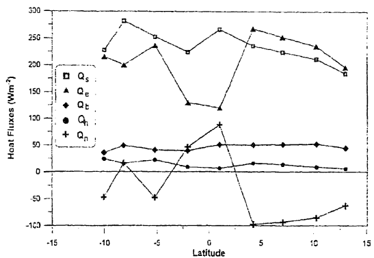
Figure 4. North-south variation of surface heat fluxes ( \text{W m}^{-2} ): shortwave radiation ( Q_s ), latent heat flux ( Q_e ), effective back radiation ( Q_b ), sensible heat flux ( Q_h ) and net heat flux ( Q_n ).
