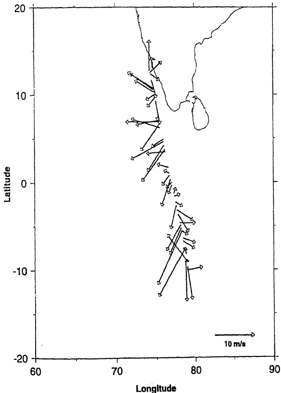
Figure 3. Distribution of surface winds along the cruise track.
