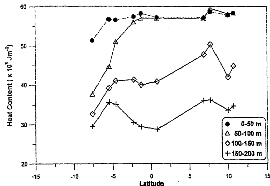
Figure 5. North-south variation of heat content ( \times 10^8 \text{ Jm}^{-2} ) in different layers.
