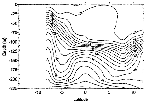
Figure 7. Vertical structure of temperature ( ^{\circ}\text{C} ) in the upper water column (0–225 m depth) along the ship's transect.
