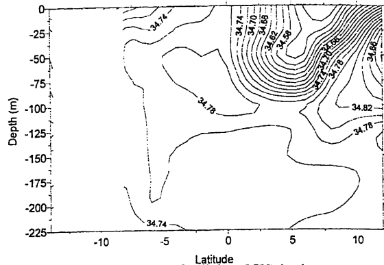
Figure 8. Vertical structure of salinity (PSU) in the upper water column (0–225 m depth) along the ship's transect.
