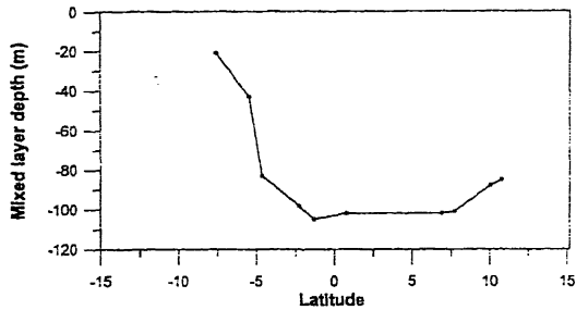
Figure 6. North-south variation of mixed layer thickness (m).
