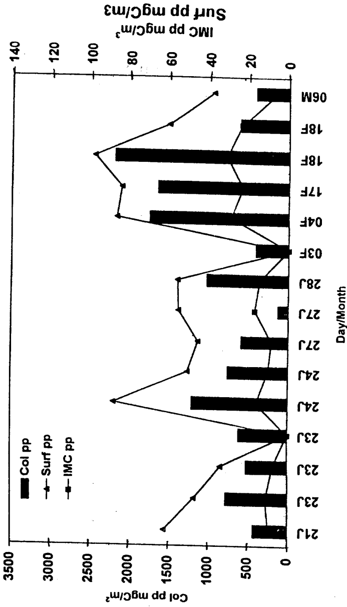
Fig.3 : Surface ( \text{mgC}/\text{m}^2/\text{d} ), column ( \text{mgC}/\text{m}^2/\text{d} ) & IM productivity values at the anchored station ( 69^{\circ}57' \text{ S} & 11^{\circ} 55' \text{ E} )
