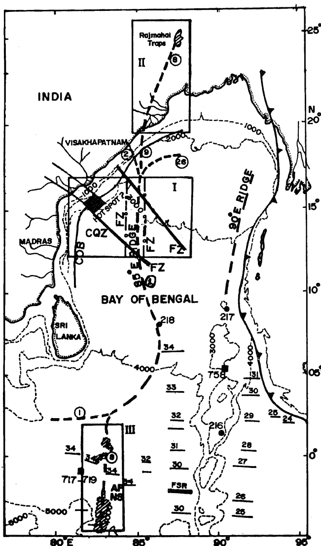
Figure 1. Northern Bengal Fan with critical areas (marked as Blocks I, II and III) where interpretations differ on seafloor spreading anomalies, fracture zones, Crozet (85°E ridge) and Marion hot spot trends 19 . Numbers in circles are references quoted in the text. COB: Continent Ocean Boundary; CQZ: Cretaceous Quiet Zone; FZ: fracture zones identified by Gopala Rao et al. 19 ; dash and dot lines are N–S fracture zones proposed from the present study. AF–NS: Afnasi–Nikitin seamounts.
