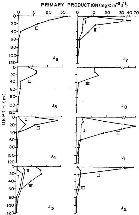
Figure 2. Primary production during the inter-monsoon (I), winter monsoon (II) and summer monsoon (III) periods.
