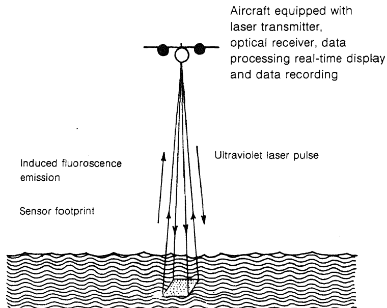
Figure 2. Laser fluorosensor operation principle. [From Soresen, 1984]
