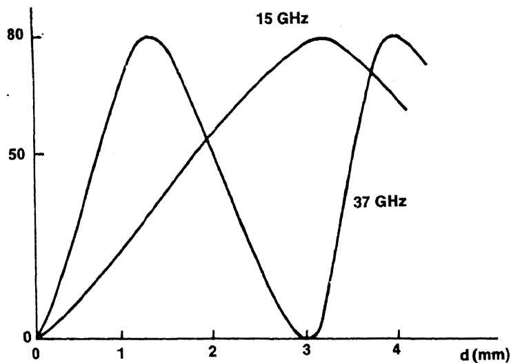
Figure 1. Changes in brightness temperature at 15 and 37 MHz for variable oil thicknesses. Vertical view. [From Soresen, 1984]
