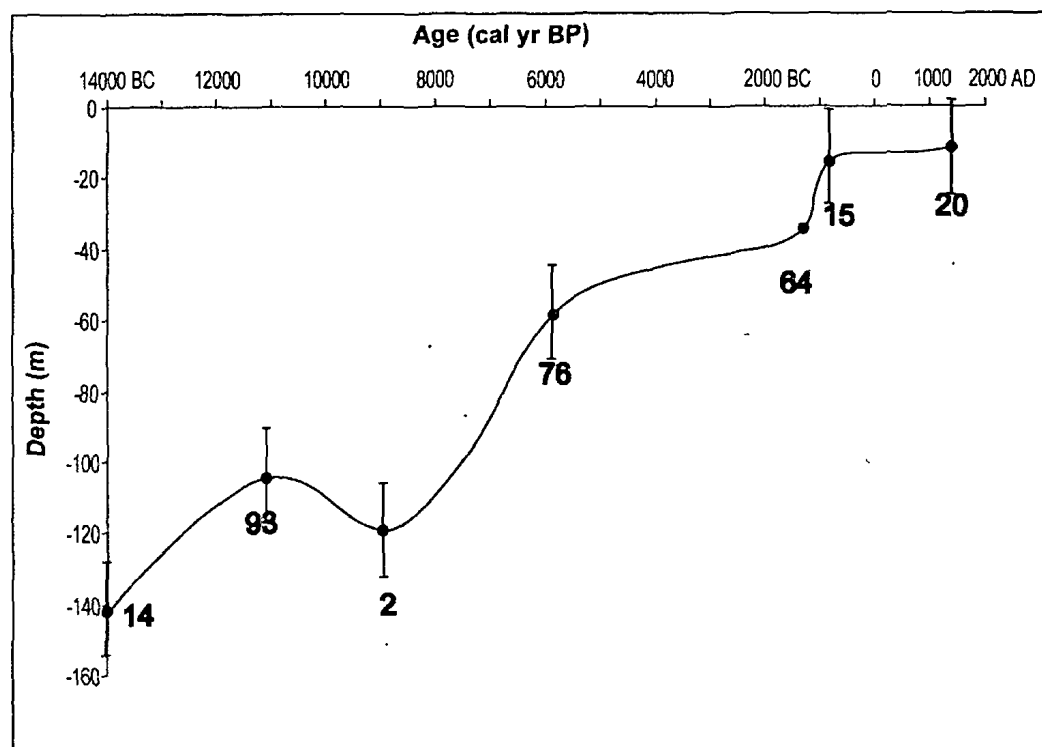
Fig 8 Sea Level Curve proposed for the West Coast of Myanmar based on the ecology of the soft coral assemblage (sample numbers indicated with corresponding numbers) and 14 C dates of relict foraminiferal assemblage
