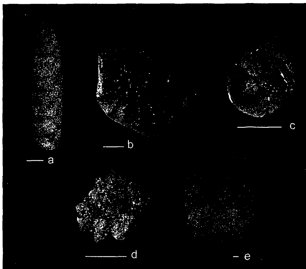
Fig. 2 Relict larger foraminiferal assemblage encountered along the west coast of Myanmar (present study); a. Alveolinella , b. Operculina , c. Amphistegina , d. Calcarina , e. Heferostegina (Scale Bar = 2000 \mu m)
