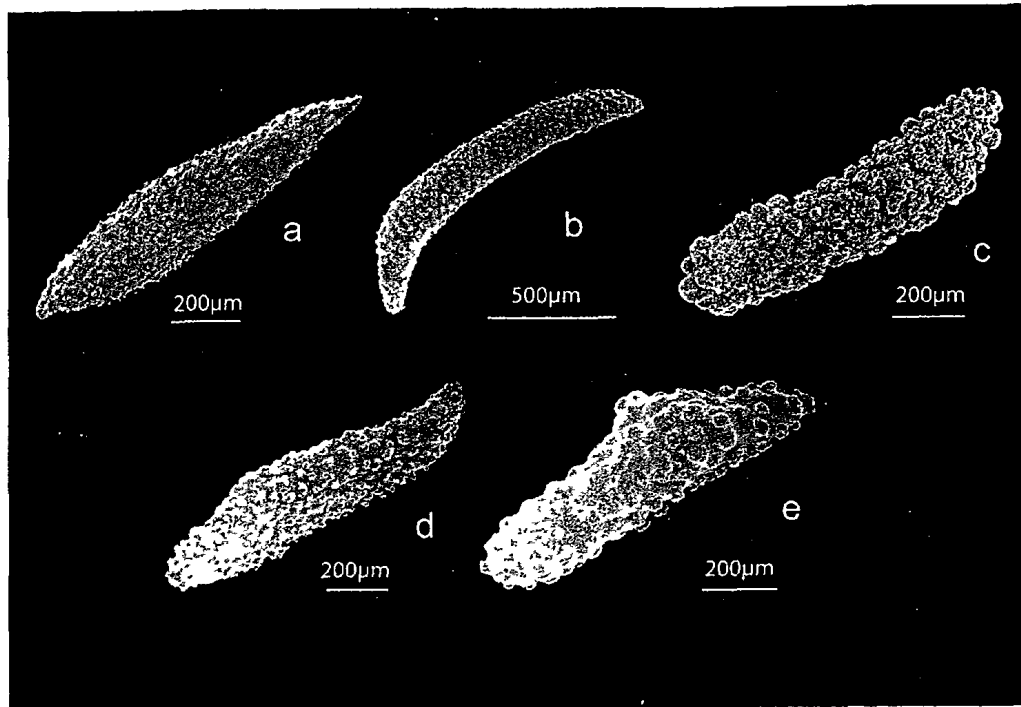
Fig 4 Selerites of the soft coral assemblage encountered during the present study a Siphonogorgia b Chronophthya c Subergorgia d Acalvoigorgia and e. Ctenocella (Scale Bar = 2000µm)
