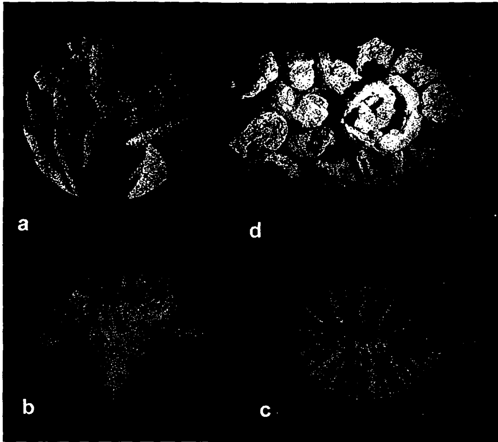
Fig. 3 Associated coral fauna; a. Microphotograph showing bulk sclerites (25x), b side view of a caryophyllid specimen (7x), c. top view of the same caryophyllid specimen; d Coral rubble and debris; transverse sections of a few specimens show the concentric growth of coralline algae
