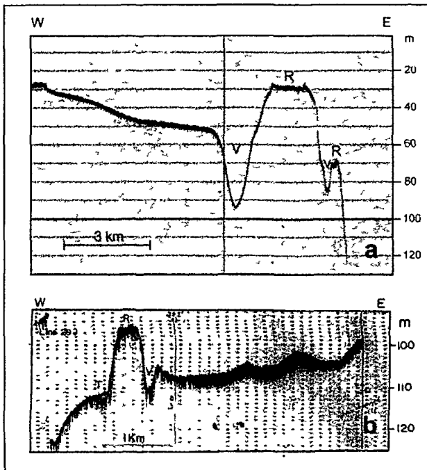
Fig 5 Comparison between E-W echograms obtained along the west coast of a Myanmar (station Hand 15 in the present study) and b India (Vora et al. 1996)
