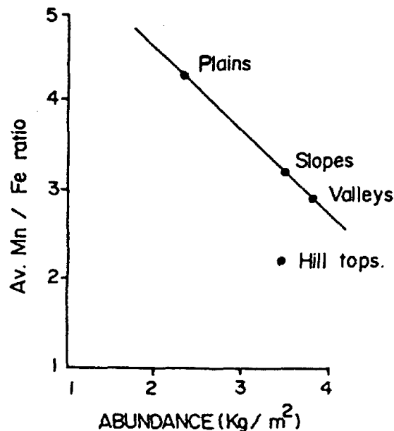
Fig.2. Relation between nodule abundance (kg/m 2 ) and Av. Mn/Fe ratio
