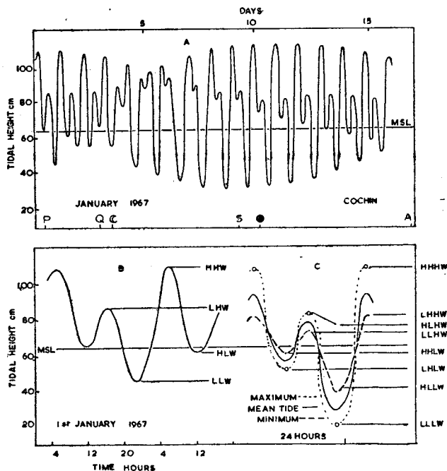
FIG. 2. (A) Tidal curve at Cochin during the first fortnight of January 1967 showing mixed, semidiurnal tides, along with phases of the moon. (B) Tidal cycle on January 1, 1967 showing two successive high and low tides. (C) Diagrammatic representation of the highest and lowest elevations of the tides in relation to mean tides. In all the figures the mean sea level (MSL) is indicated by a horizontal line at about 64 cm.
