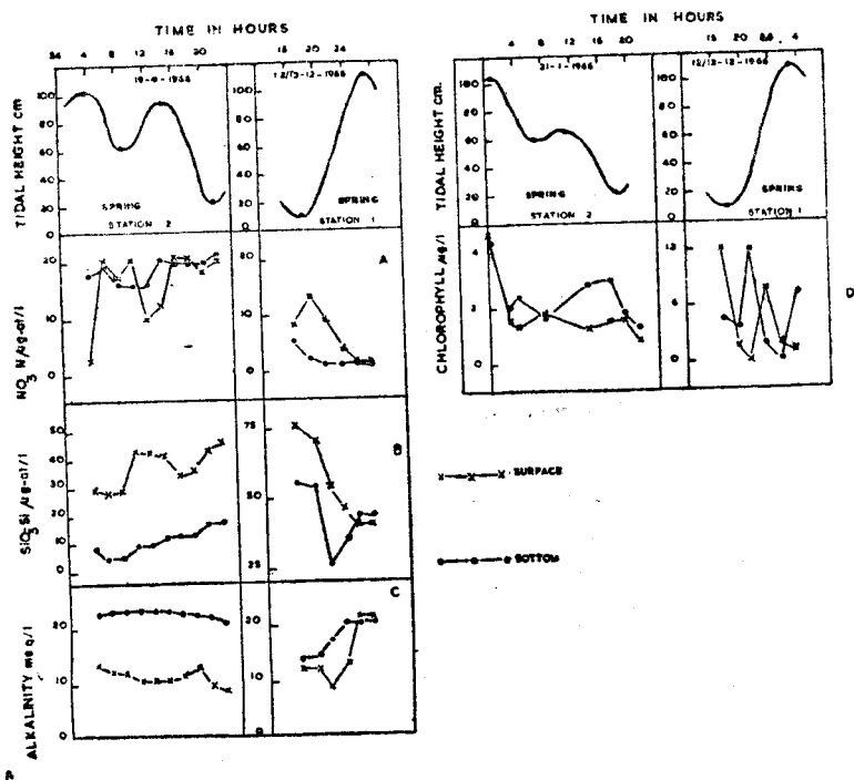
FIG. 5. Changes in nitrate-N (A), silicate-Si (B), alkalinity (C), and chlorophyll (D), at the surface and bottom, during the tidal cycles. The top drawings represent the tidal curves.
