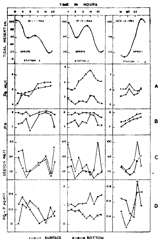
FIG. 4. Changes in dissolved oxygen (A), pH (B), seston (C), and phosphorus (D), at the surface and bottom, during the tidal cycles. The top drawings represent the tidal curves.
