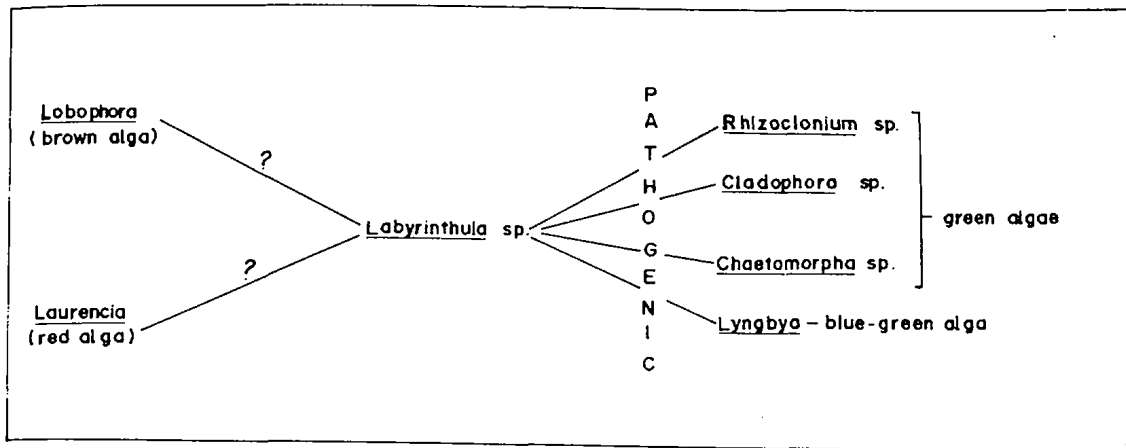
Fig. 36. Labyrinthula sp. Schematic diagram showing the host range
