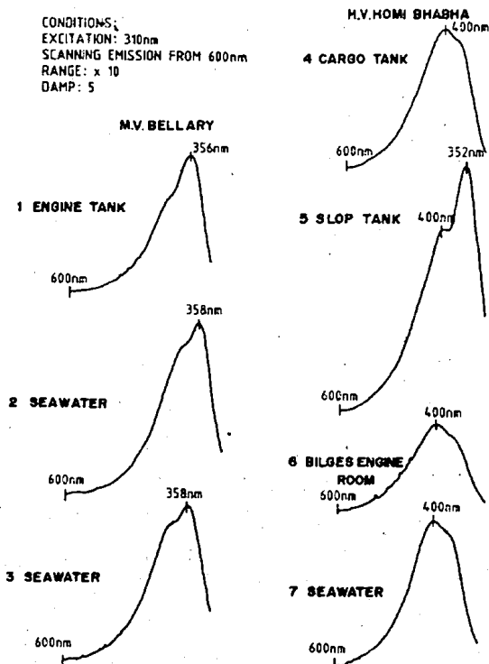
Fig. 3 – UV fluorescence spectra of samples
