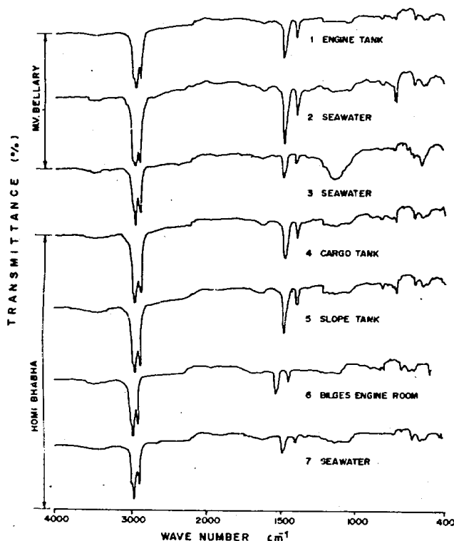
Fig. 2 – IR spectra of samples
