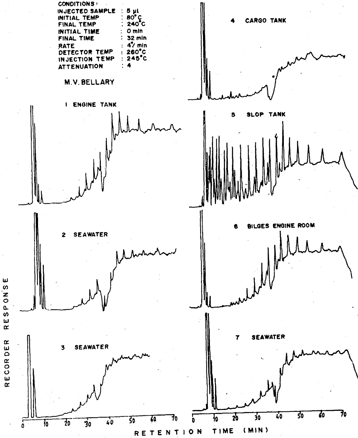
Fig. 1 - Gas chromatograms of samples
