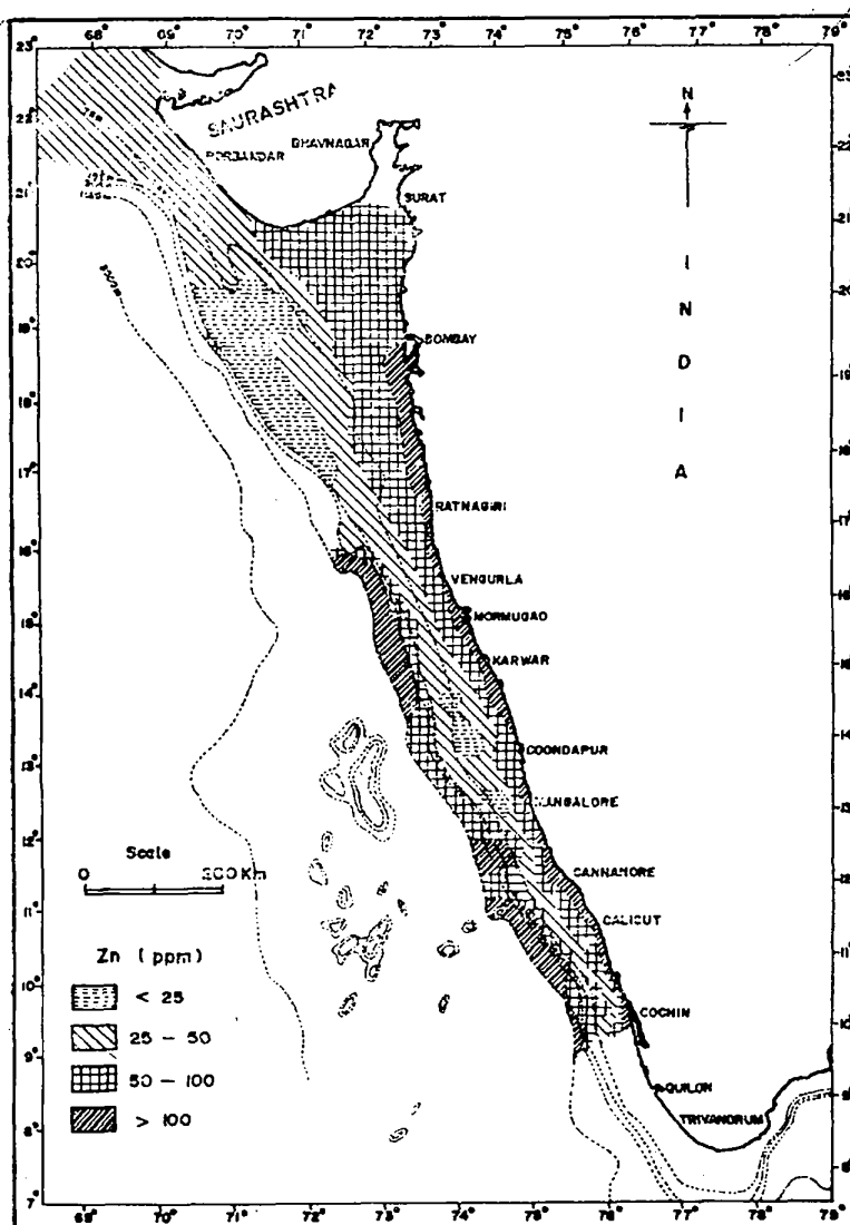
Fig. 1. Map showing the distribution of Zinc.
