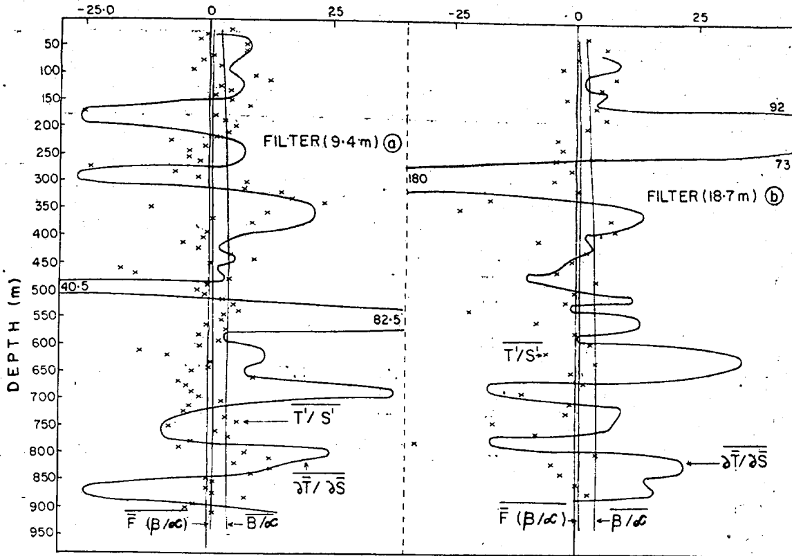
Figs. 5 (a&b) . A comparative evaluation of \beta/\alpha , T'/S' and \partial\bar{T}/\partial\bar{S} at station 167
