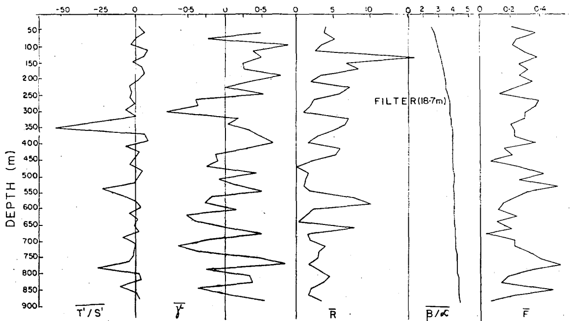
Fig. 6. Vertical structure of averaged (over 18.7 m) statistics computed from data filtered using a Cosine filter (18.7 m)
