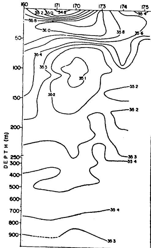
Fig. 3. Vertical salinity structure along the latitudinal section
