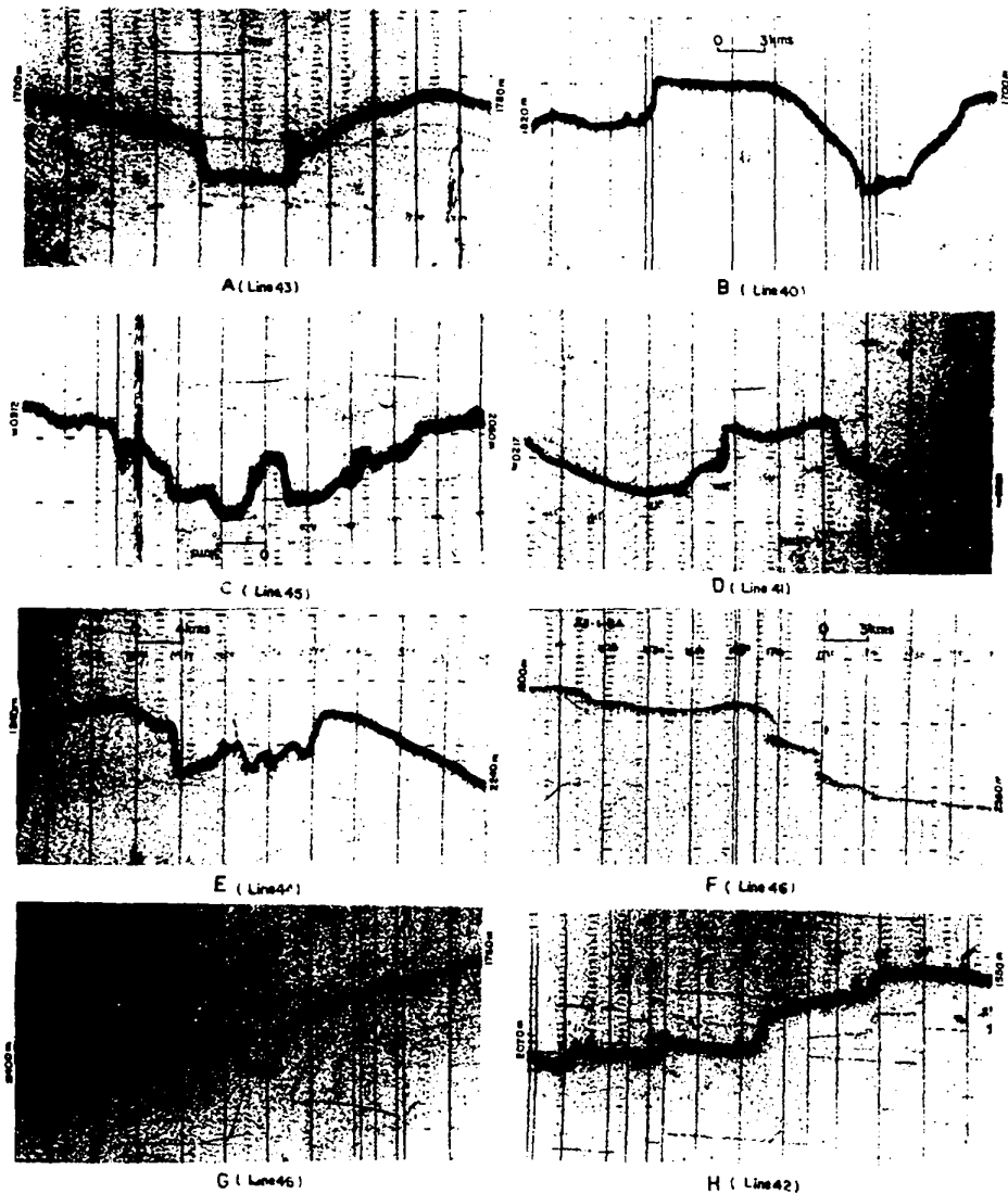
Fig. 4.: Echograms of the seabed showing, scarps/faults, canyons and valleys/graben.
