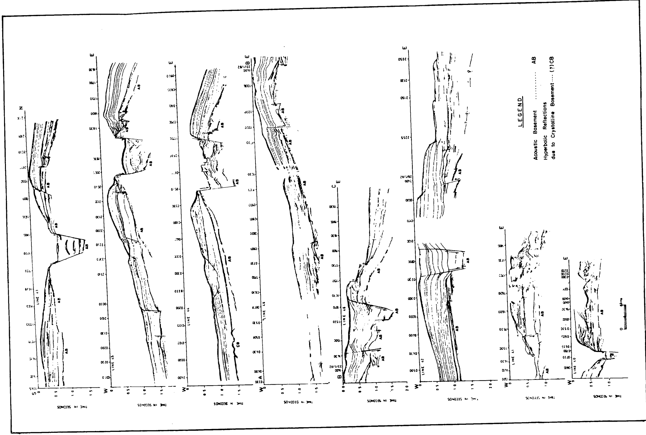
Fig. 5. Seismic reflection profiles over the Astrid Ridge. Two ways travel time in seconds, acoustic basement (AB), and crystalline basement (CB) are indicated.
