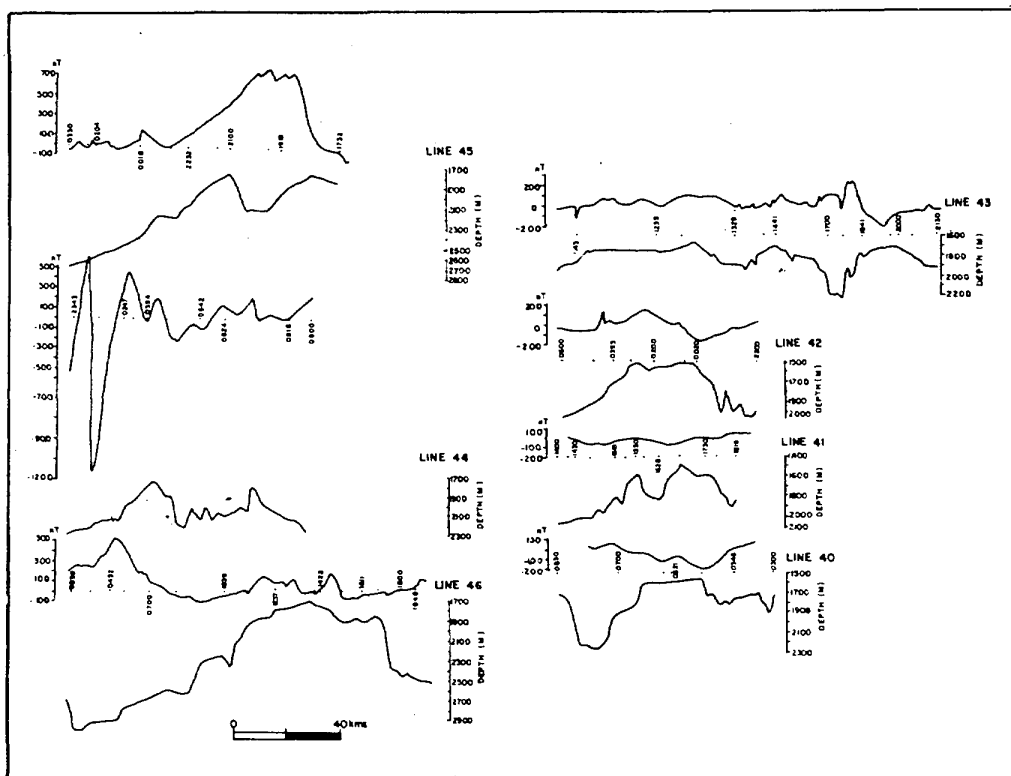
Fig.9 Topography of the sea bed and total intensity residual magnetic anomalies along the lines surveyed.
