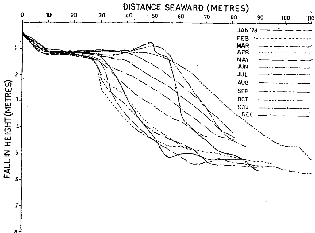
Fig. 6. Changes in beach levels at Station 9.
