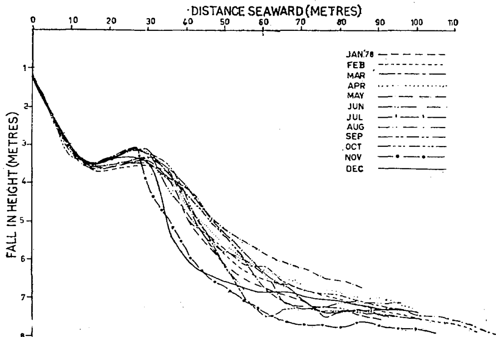
Fig. 4. Changes in beach levels at Station 13.
