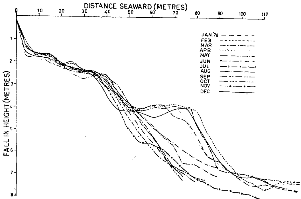
Fig. 5. Changes in beach levels at Station 11.
