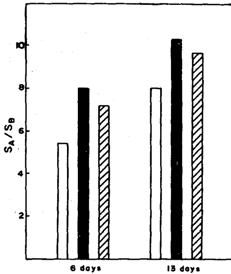
Figure 4. Ratio of areas covered by spectral peaks A and B of 90% acetone extracts of Dunaliella cells grown for 6 and 13 days in media containing NaCl at concentrations of 0.5 M (□), 1 M (■) and 2 M (▨).
