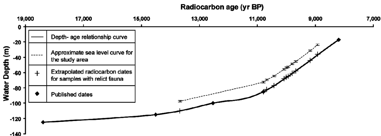
Fig. 3—Age-Depth relationship curve for the study area constructed on the basis of 5 published dates: Vaz 21,22 ; Rao et al. 8 and Mohana Rao & Rao 9 . Dotted line represents pliable sea level curve during ~ 13,600-8,900 years BP as derived from extrapolating the dates for the samples containing relict fauna.
