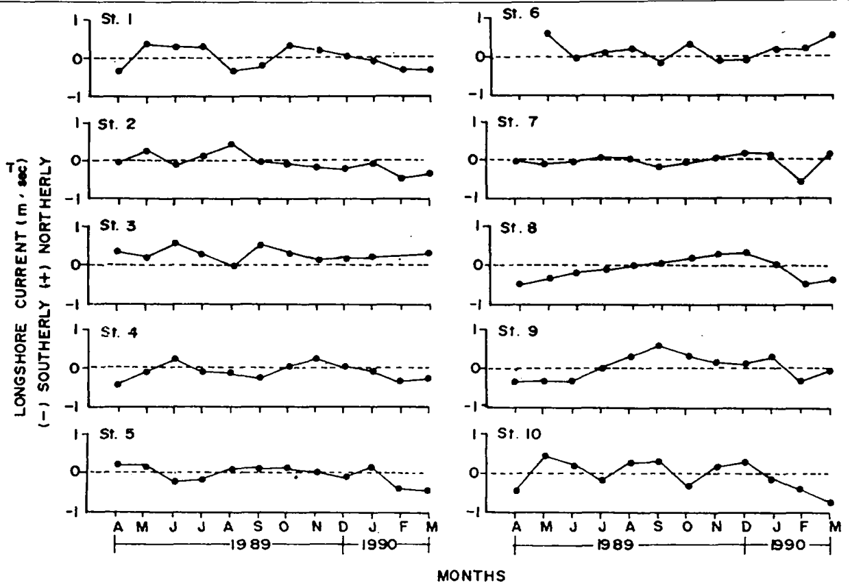
Fig. 4—Monthly longshore current distribution
