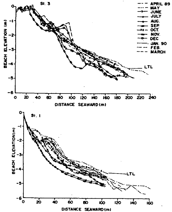
Fig. 2—Beach level variation at sts 1 and 3
