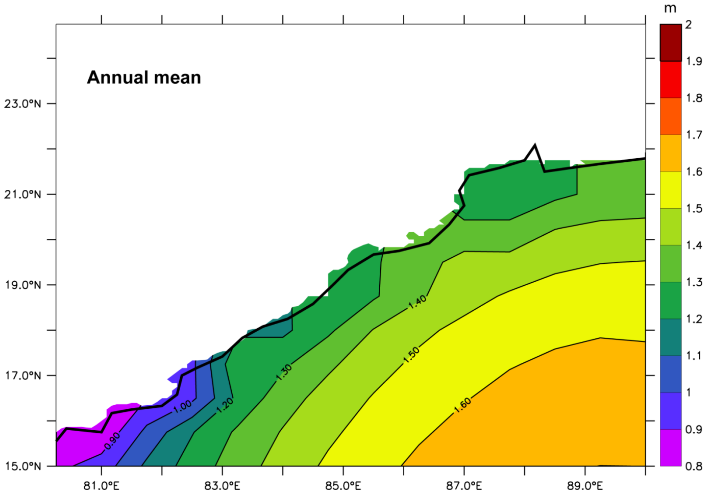
Fig.6 Map of annual Significant Wave Height (SWH)
