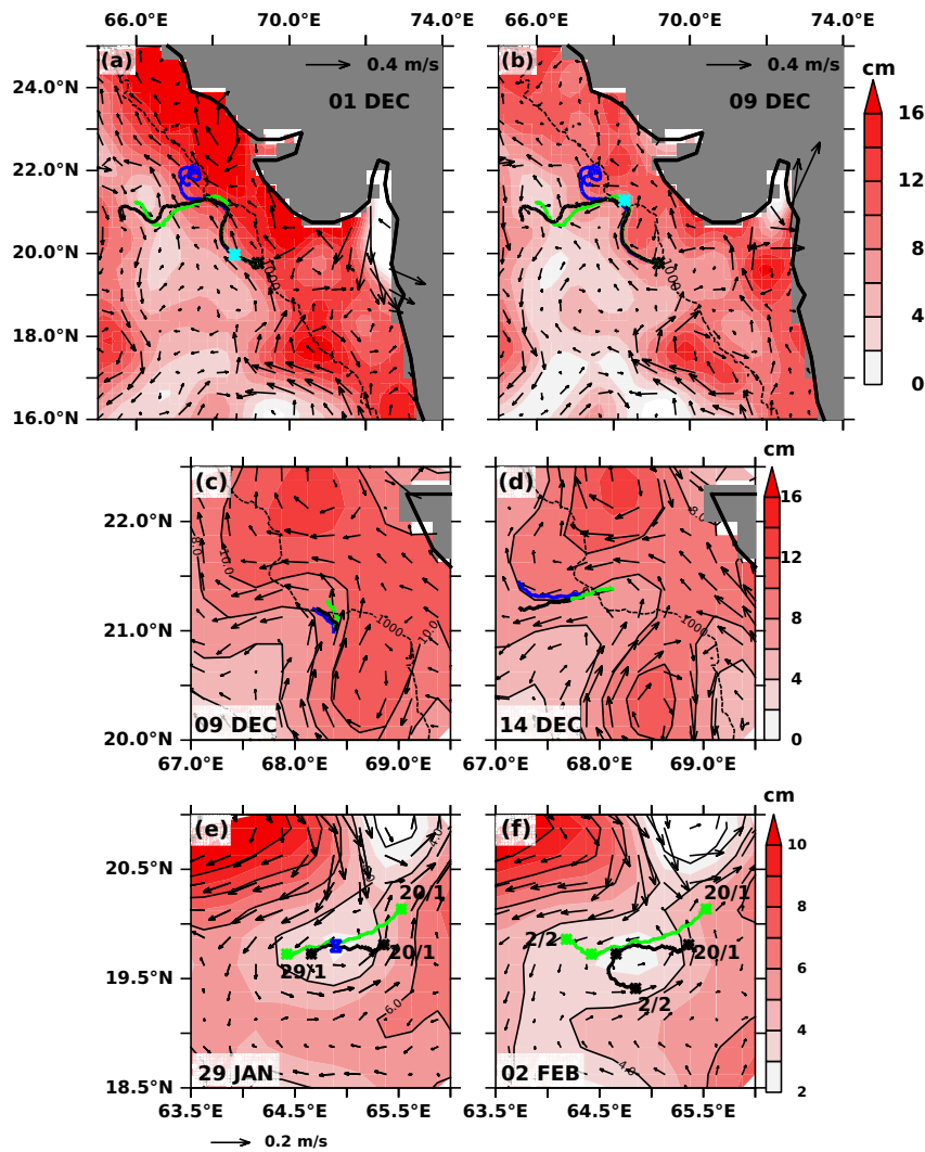
Figure 2: SLA with drifter trajectories. The overlaid vectors show the geostrophic currents. (a) SLA on 01 December 2016 with trajectories of drifters D1, D2 and D3 from 29 November 2016 to 31 December 2016; cyan star represents position of drifters on 01 December 2016. (b) Same as (a) but for 09 December 2016, (c) SLA on 09 December 2016 with drifters trajectories from 08–09 December 2016, (d) SLA on 14 December 2016 with drifters trajectories from 08–09 December 2016, (e) SLA on 29 January 2017 with drifters trajectories from 20–29 January 2017; 20 January 2017 and 29 January 2017 are denoted by black stars, blue cross represents 28 January 2017, (f) SLA on 02 February 2017 with drifters trajectories from 20 January 2017 to 02 February 2017. In panels (a)-(d), the dashed black line represents 1000 m contour.
