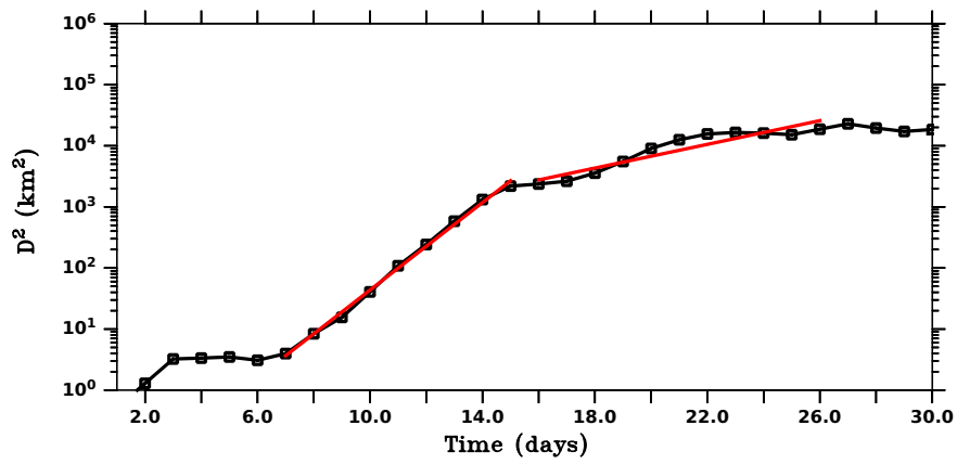
Figure 3: Relative dispersion on a semi-logarithmic graph. Red lines shows exponential fit for 7-15 and 16-26 days respectively.
